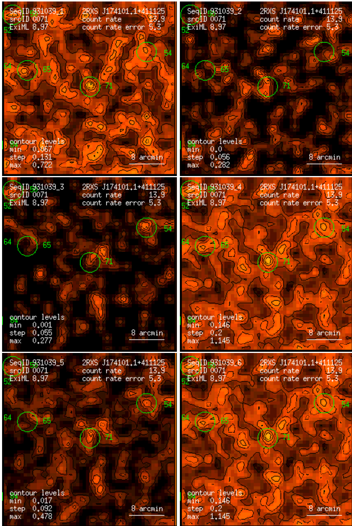
Figure 71: RASS 931039: detection 0071: band rate images, Gaussian filter: (1) PSPC channels 11 – 41, (2) 52 – 90, (3) 91 – 201, (4) 11 – 235, (5) 52 – 201, (6) 11 – 201. Broad band rates in counts/ks. Band rate contour levels in counts/ks/arcmin 2 .
