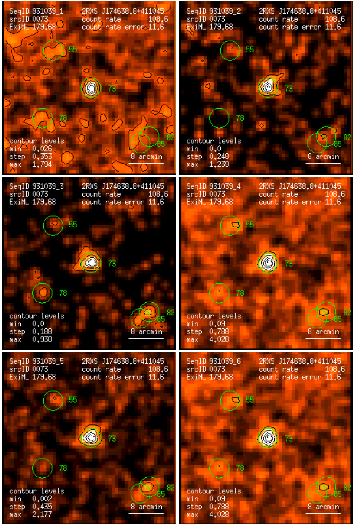
Figure 73: RASS 931039: detection 0073: band rate images, Gaussian filter: (1) PSPC channels 11 – 41, (2) 52 – 90, (3) 91 – 201, (4) 11 – 235, (5) 52 – 201, (6) 11 – 201. Broad band rates in counts/ks. Band rate contour levels in counts/ks/arcmin 2 .
