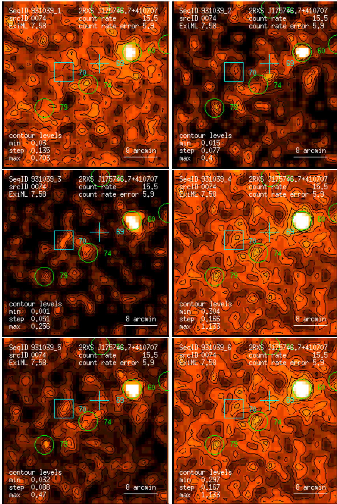
Figure 74: RASS 931039: detection 0074: band rate images, Gaussian filter: (1) PSPC channels 11 – 41, (2) 52 – 90, (3) 91 – 201, (4) 11 – 235, (5) 52 – 201, (6) 11 – 201. Broad band rates in counts/ks. Band rate contour levels in counts/ks/arcmin 2 .
