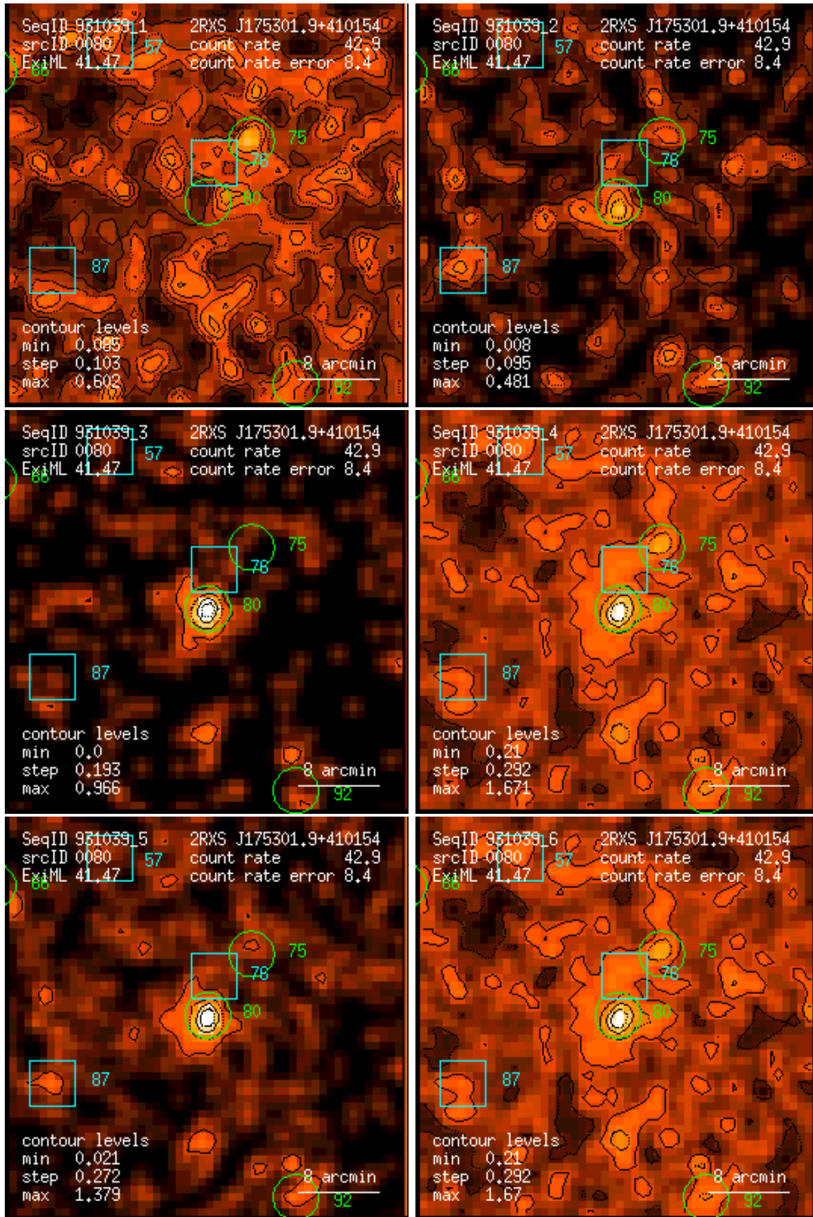
Figure 80: RASS 931039: detection 0080: band rate images, Gaussian filter: (1) PSPC channels 11 – 41, (2) 52 – 90, (3) 91 – 201, (4) 11 – 235, (5) 52 – 201, (6) 11 – 201. Broad band rates in counts/ks. Band rate contour levels in counts/ks/arcmin 2 .
