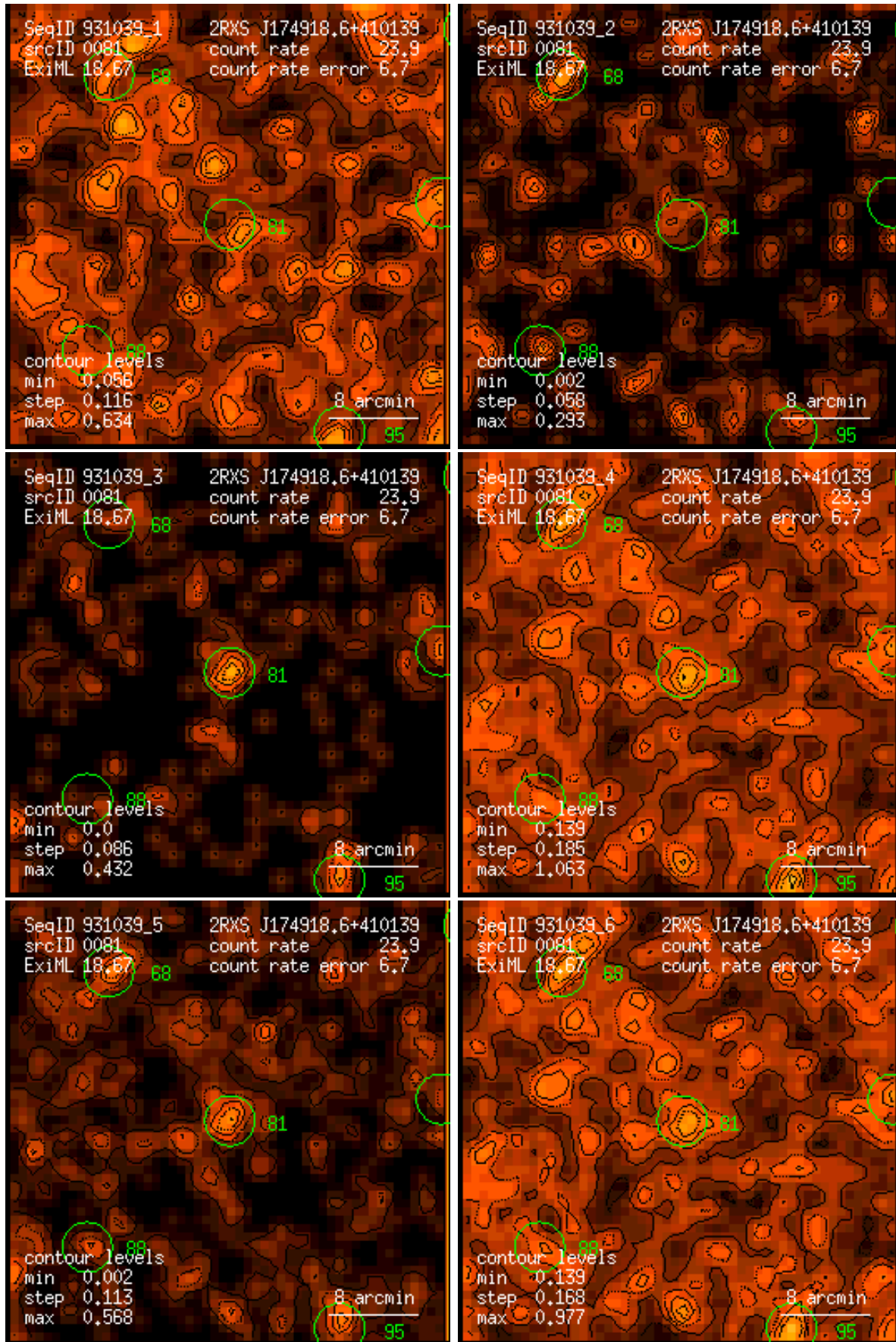
Figure 81: RASS 931039: detection 0081: band rate images, Gaussian filter: (1) PSPC channels 11 – 41, (2) 52 – 90, (3) 91 – 201, (4) 11 – 235, (5) 52 – 201, (6) 11 – 201. Broad band rates in counts/ks. Band rate contour levels in counts/ks/arcmin 2 .
