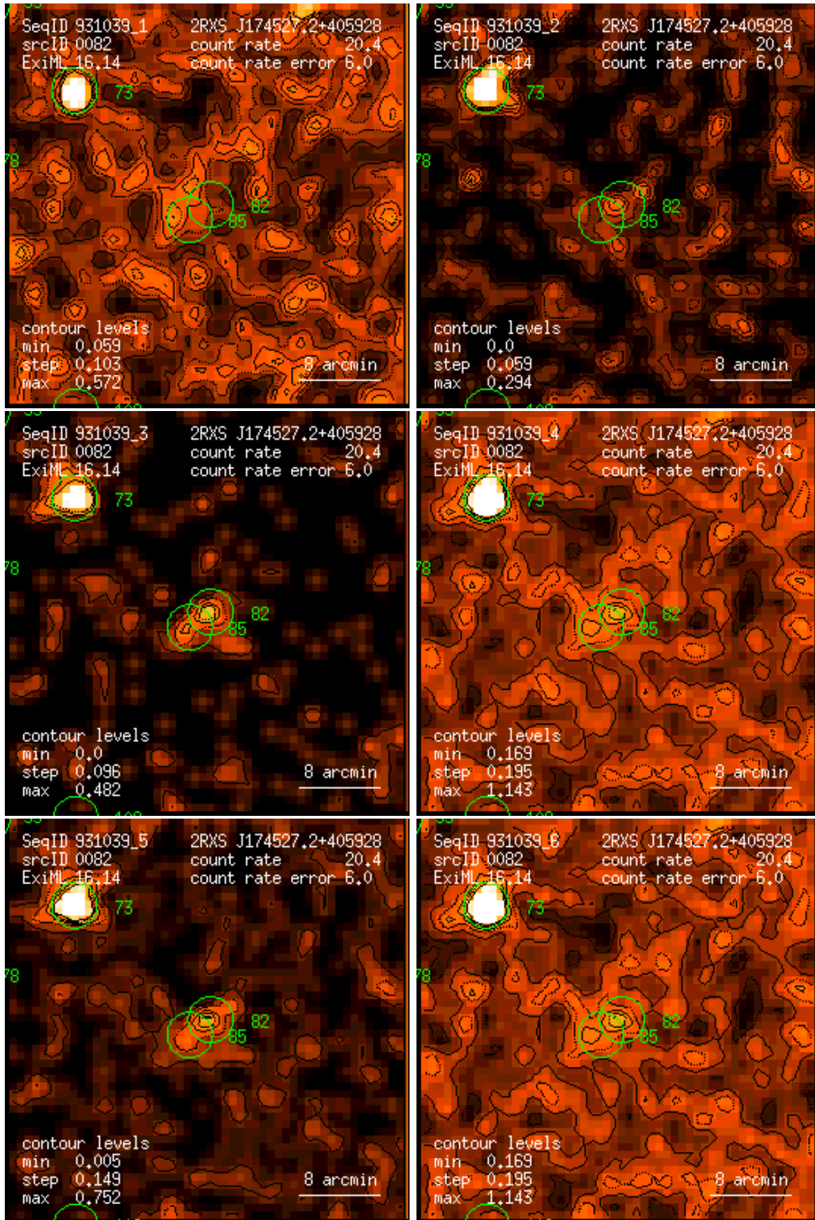
Figure 82: RASS 931039: detection 0082: band rate images, Gaussian filter: (1) PSPC channels 11 – 41, (2) 52 – 90, (3) 91 – 201, (4) 11 – 235, (5) 52 – 201, (6) 11 – 201. Broad band rates in counts/ks. Band rate contour levels in counts/ks/arcmin 2 .
