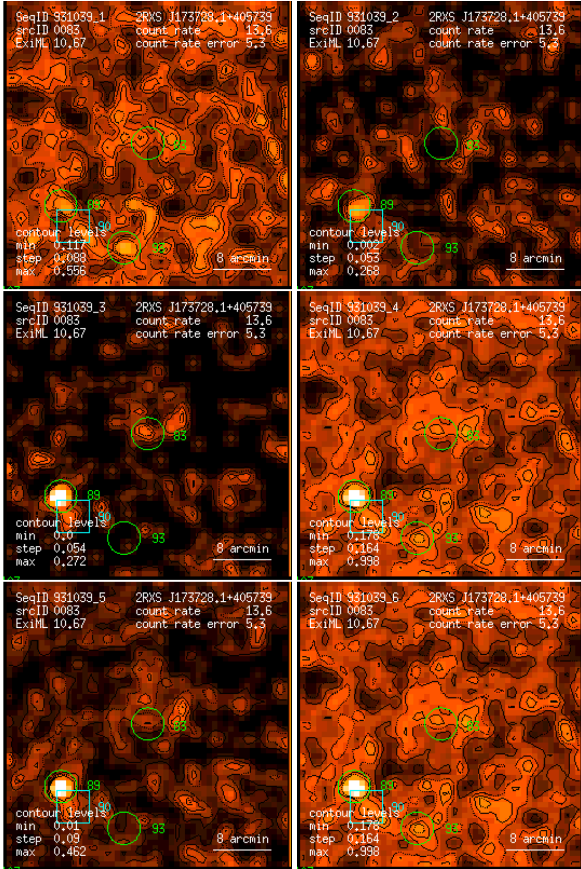
Figure 83: RASS 931039: detection 0083: band rate images, Gaussian filter: (1) PSPC channels 11 – 41, (2) 52 – 90, (3) 91 – 201, (4) 11 – 235, (5) 52 – 201, (6) 11 – 201. Broad band rates in counts/ks. Band rate contour levels in counts/ks/arcmin 2 .
