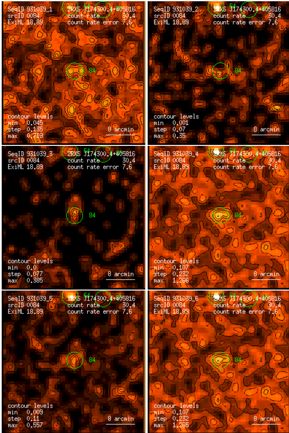
Figure 84: RASS 931039: detection 0084: band rate images, Gaussian filter: (1) PSPC channels 11 – 41, (2) 52 – 90, (3) 91 – 201, (4) 11 – 235, (5) 52 – 201, (6) 11 – 201. Broad band rates in counts/ks. Band rate contour levels in counts/ks/arcmin 2 .
