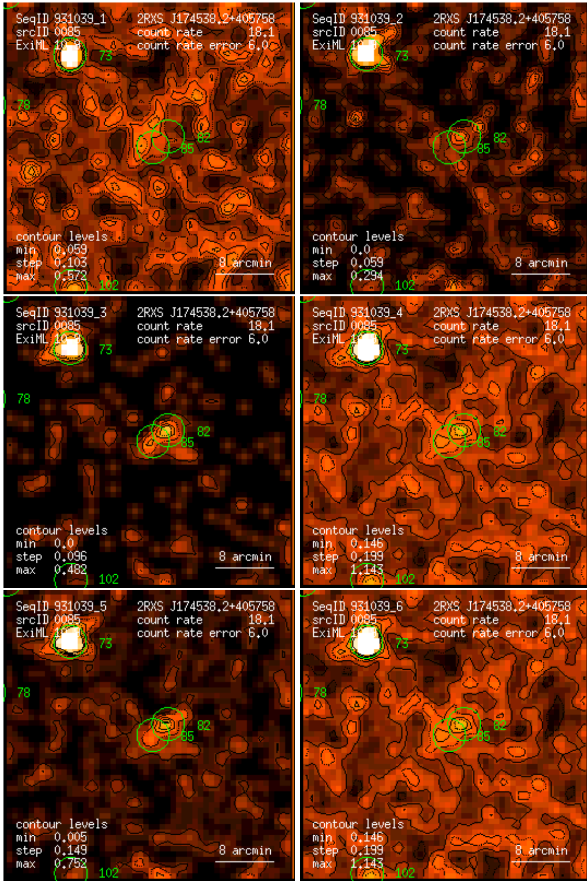
Figure 85: RASS 931039: detection 0085: band rate images, Gaussian filter: (1) PSPC channels 11 – 41, (2) 52 – 90, (3) 91 – 201, (4) 11 – 235, (5) 52 – 201, (6) 11 – 201. Broad band rates in counts/ks. Band rate contour levels in counts/ks/arcmin 2 .
