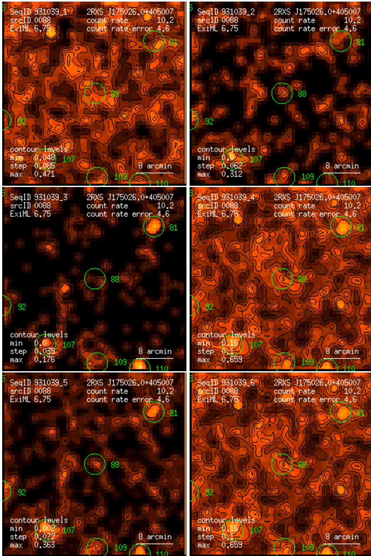
Figure 88: RASS 931039: detection 0088: band rate images, Gaussian filter: (1) PSPC channels 11 – 41, (2) 52 – 90, (3) 91 – 201, (4) 11 – 235, (5) 52 – 201, (6) 11 – 201. Broad band rates in counts/ks. Band rate contour levels in counts/ks/arcmin 2 .
