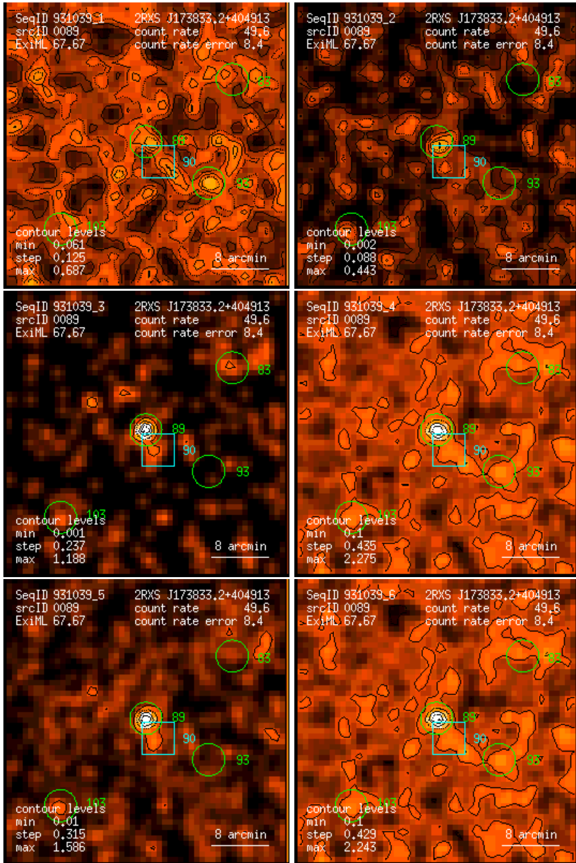
Figure 89: RASS 931039: detection 0089: band rate images, Gaussian filter: (1) PSPC channels 11 – 41, (2) 52 – 90, (3) 91 – 201, (4) 11 – 235, (5) 52 – 201, (6) 11 – 201. Broad band rates in counts/ks. Band rate contour levels in counts/ks/arcmin 2 .
