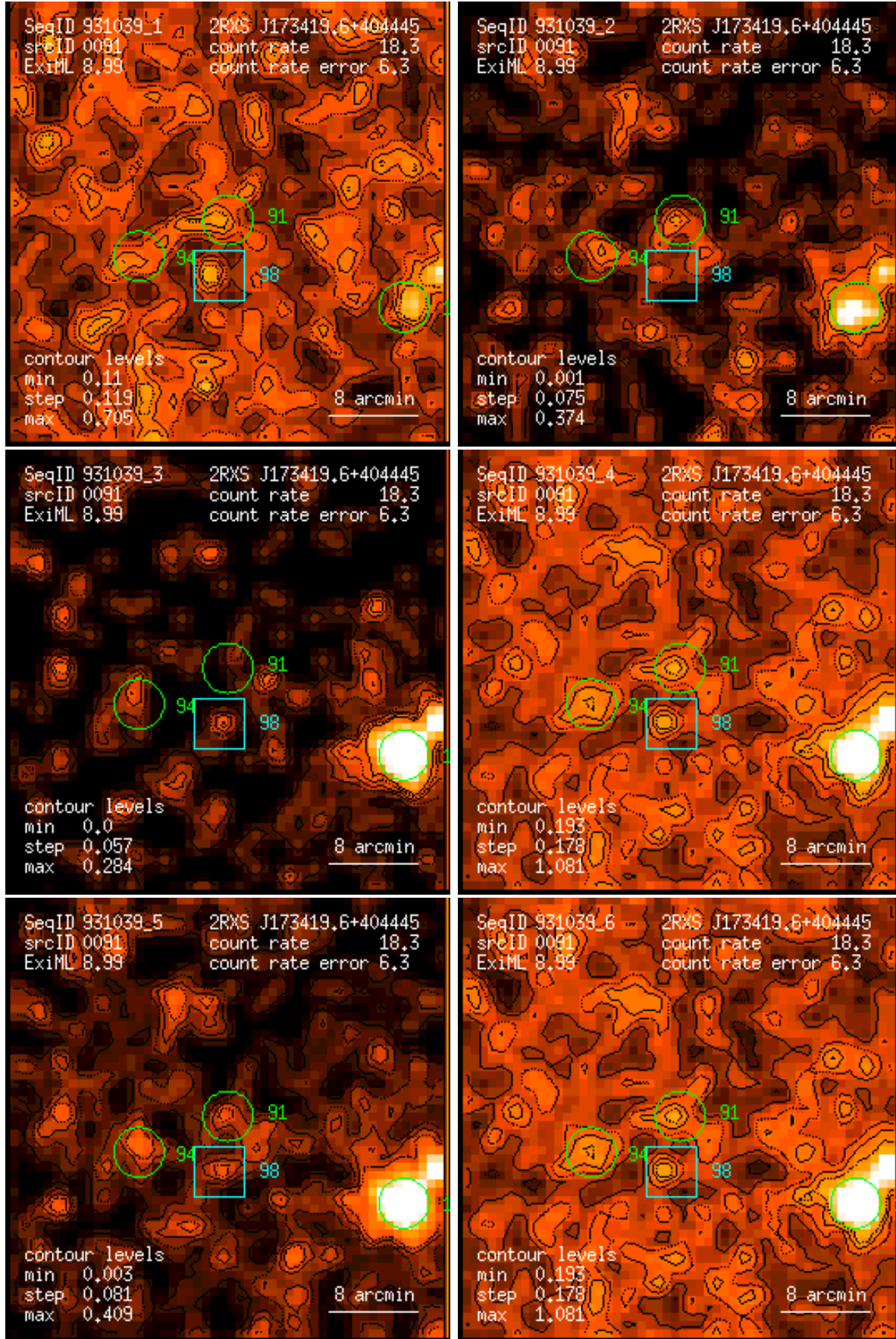
Figure 91: RASS 931039: detection 0091: band rate images, Gaussian filter: (1) PSPC channels 11 – 41, (2) 52 – 90, (3) 91 – 201, (4) 11 – 235, (5) 52 – 201, (6) 11 – 201. Broad band rates in counts/ks. Band rate contour levels in counts/ks/arcmin 2 .
