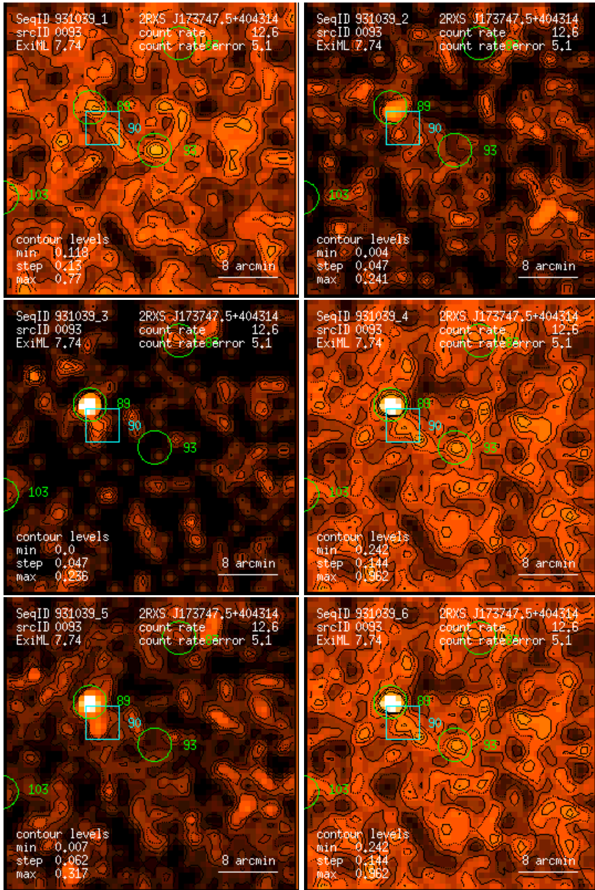
Figure 93: RASS 931039: detection 0093: band rate images, Gaussian filter: (1) PSPC channels 11 – 41, (2) 52 – 90, (3) 91 – 201, (4) 11 – 235, (5) 52 – 201, (6) 11 – 201. Broad band rates in counts/ks. Band rate contour levels in counts/ks/arcmin 2 .
