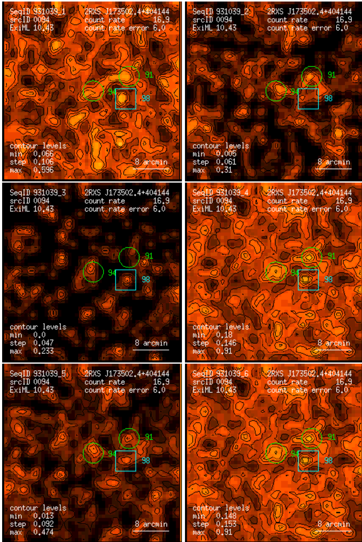
Figure 94: RASS 931039: detection 0094: band rate images, Gaussian filter: (1) PSPC channels 11 – 41, (2) 52 – 90, (3) 91 – 201, (4) 11 – 235, (5) 52 – 201, (6) 11 – 201. Broad band rates in counts/ks. Band rate contour levels in counts/ks/arcmin 2 .
