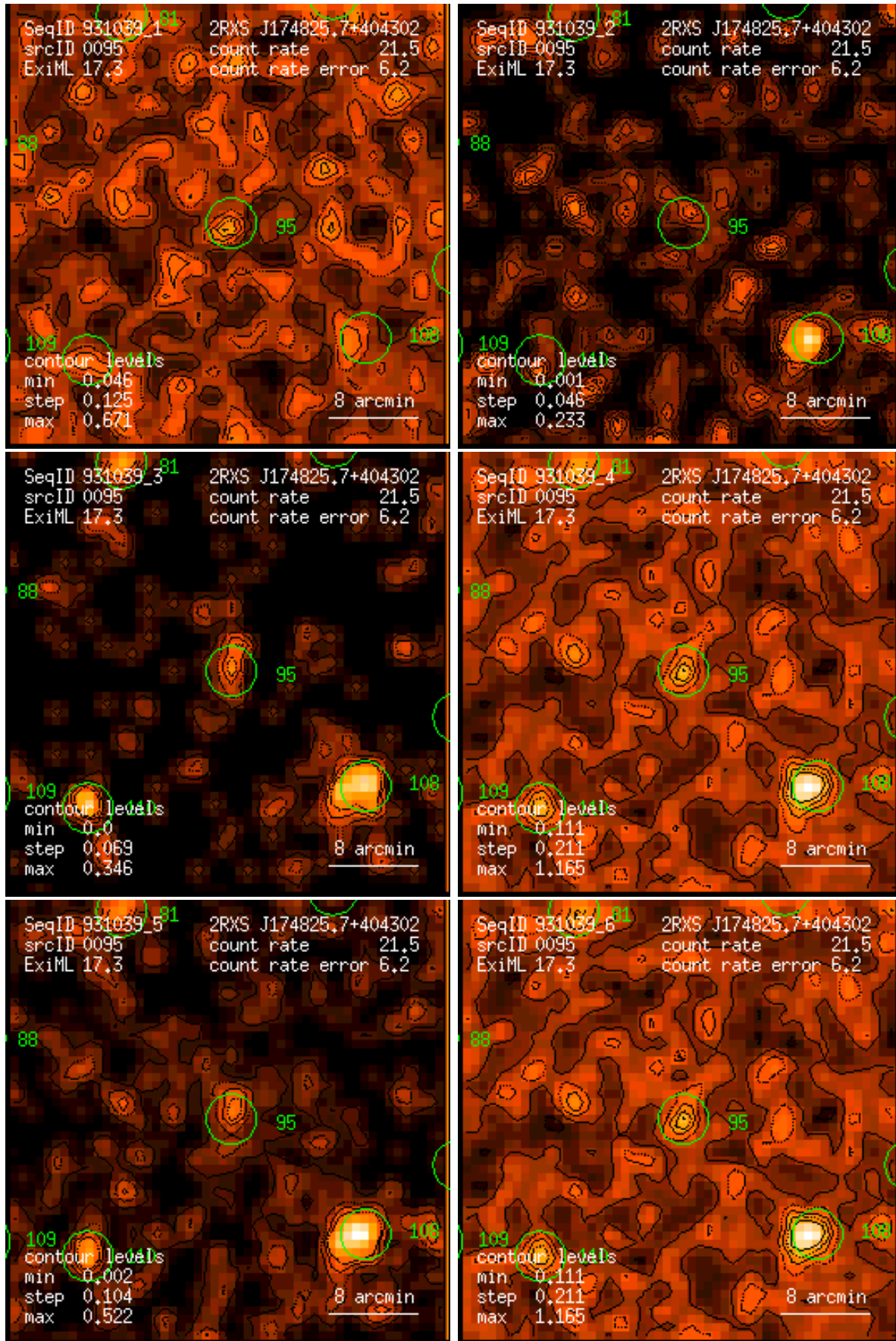
Figure 95: RASS 931039: detection 0095: band rate images, Gaussian filter: (1) PSPC channels 11 – 41, (2) 52 – 90, (3) 91 – 201, (4) 11 – 235, (5) 52 – 201, (6) 11 – 201. Broad band rates in counts/ks. Band rate contour levels in counts/ks/arcmin 2 .
