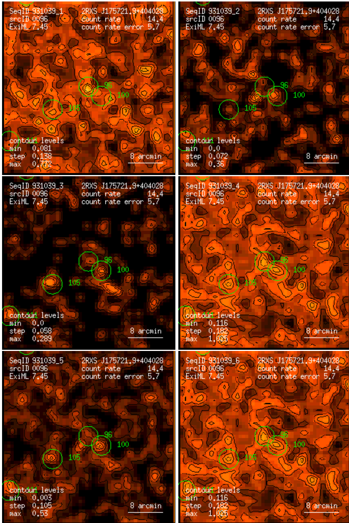
Figure 96: RASS 931039: detection 0096: band rate images, Gaussian filter: (1) PSPC channels 11 – 41, (2) 52 – 90, (3) 91 – 201, (4) 11 – 235, (5) 52 – 201, (6) 11 – 201. Broad band rates in counts/ks. Band rate contour levels in counts/ks/arcmin 2 .
