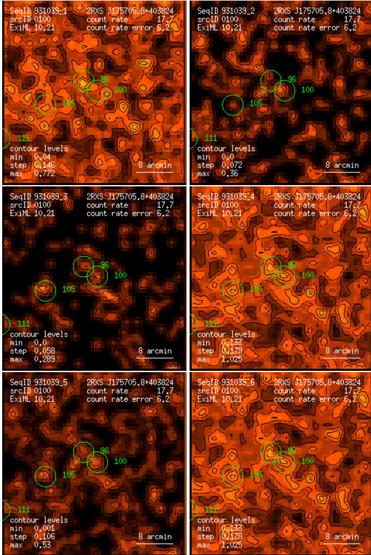
Figure 100: RASS 931039: detection 0100: band rate images, Gaussian filter: (1) PSPC channels 11 – 41, (2) 52 – 90, (3) 91 – 201, (4) 11 – 235, (5) 52 – 201, (6) 11 – 201. Broad band rates in counts/ks. Band rate contour levels in counts/ks/arcmin 2 .
