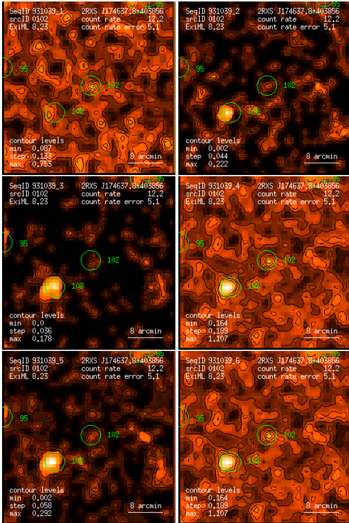
Figure 102: RASS 931039: detection 0102: band rate images, Gaussian filter: (1) PSPC channels 11 – 41, (2) 52 – 90, (3) 91 – 201, (4) 11 – 235, (5) 52 – 201, (6) 11 – 201. Broad band rates in counts/ks. Band rate contour levels in counts/ks/arcmin 2 .
