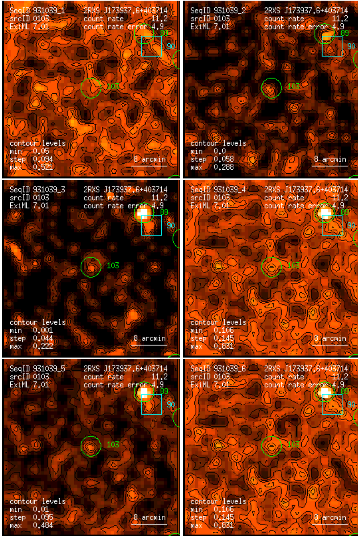
Figure 103: RASS 931039: detection 0103: band rate images, Gaussian filter: (1) PSPC channels 11 – 41, (2) 52 – 90, (3) 91 – 201, (4) 11 – 235, (5) 52 – 201, (6) 11 – 201. Broad band rates in counts/ks. Band rate contour levels in counts/ks/arcmin 2 .
