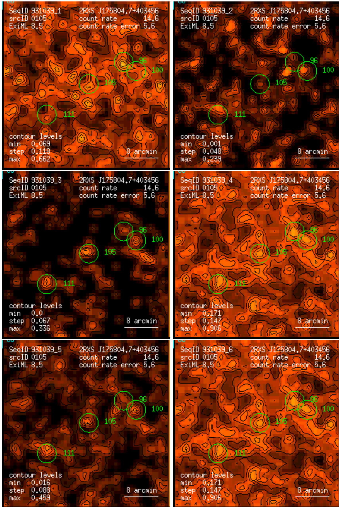
Figure 105: RASS 931039: detection 0105: band rate images, Gaussian filter: (1) PSPC channels 11 – 41, (2) 52 – 90, (3) 91 – 201, (4) 11 – 235, (5) 52 – 201, (6) 11 – 201. Broad band rates in counts/ks. Band rate contour levels in counts/ks/arcmin 2 .
