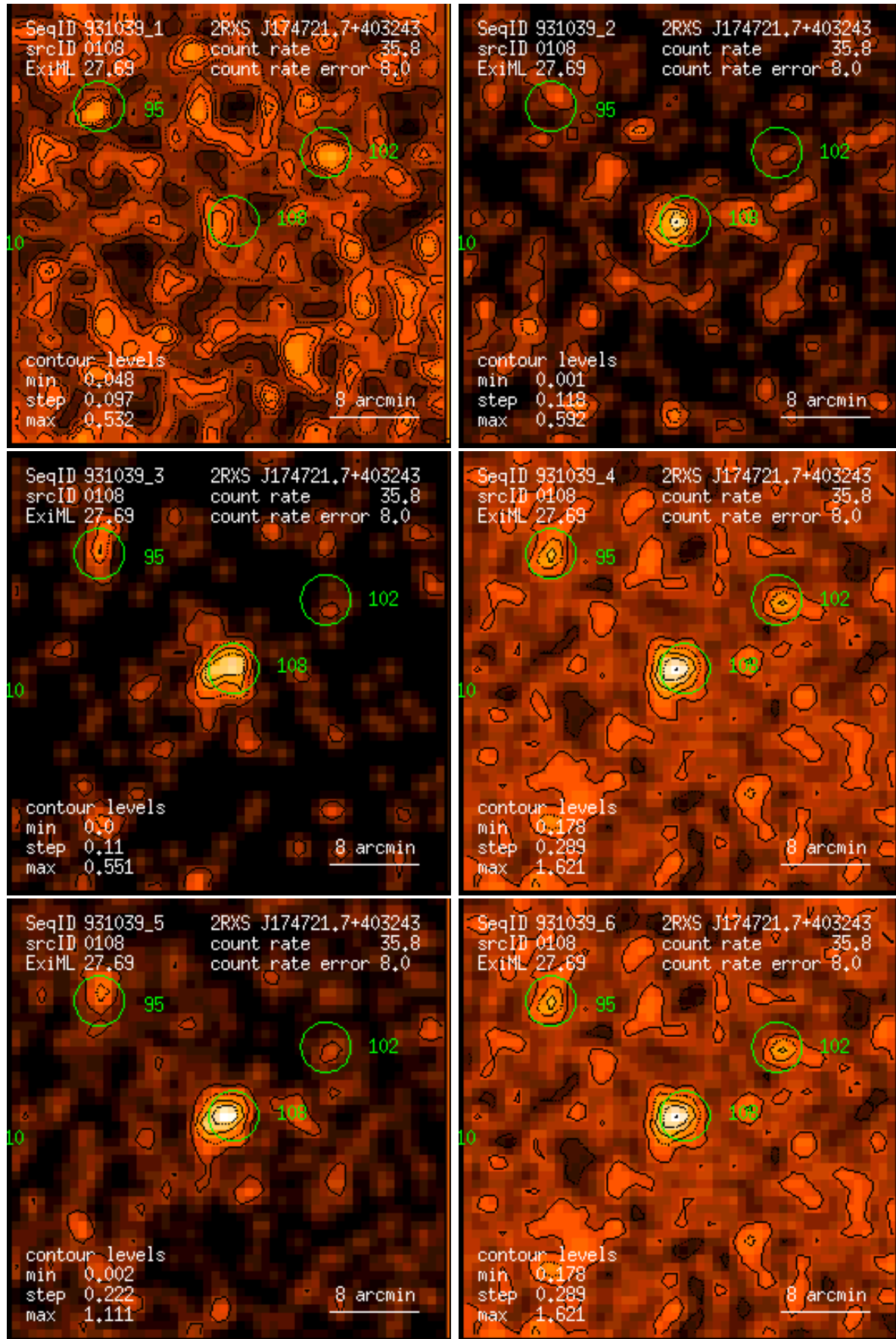
Figure 108: RASS 931039: detection 0108: band rate images, Gaussian filter: (1) PSPC channels 11 – 41, (2) 52 – 90, (3) 91 – 201, (4) 11 – 235, (5) 52 – 201, (6) 11 – 201. Broad band rates in counts/ks. Band rate contour levels in counts/ks/arcmin 2 .
