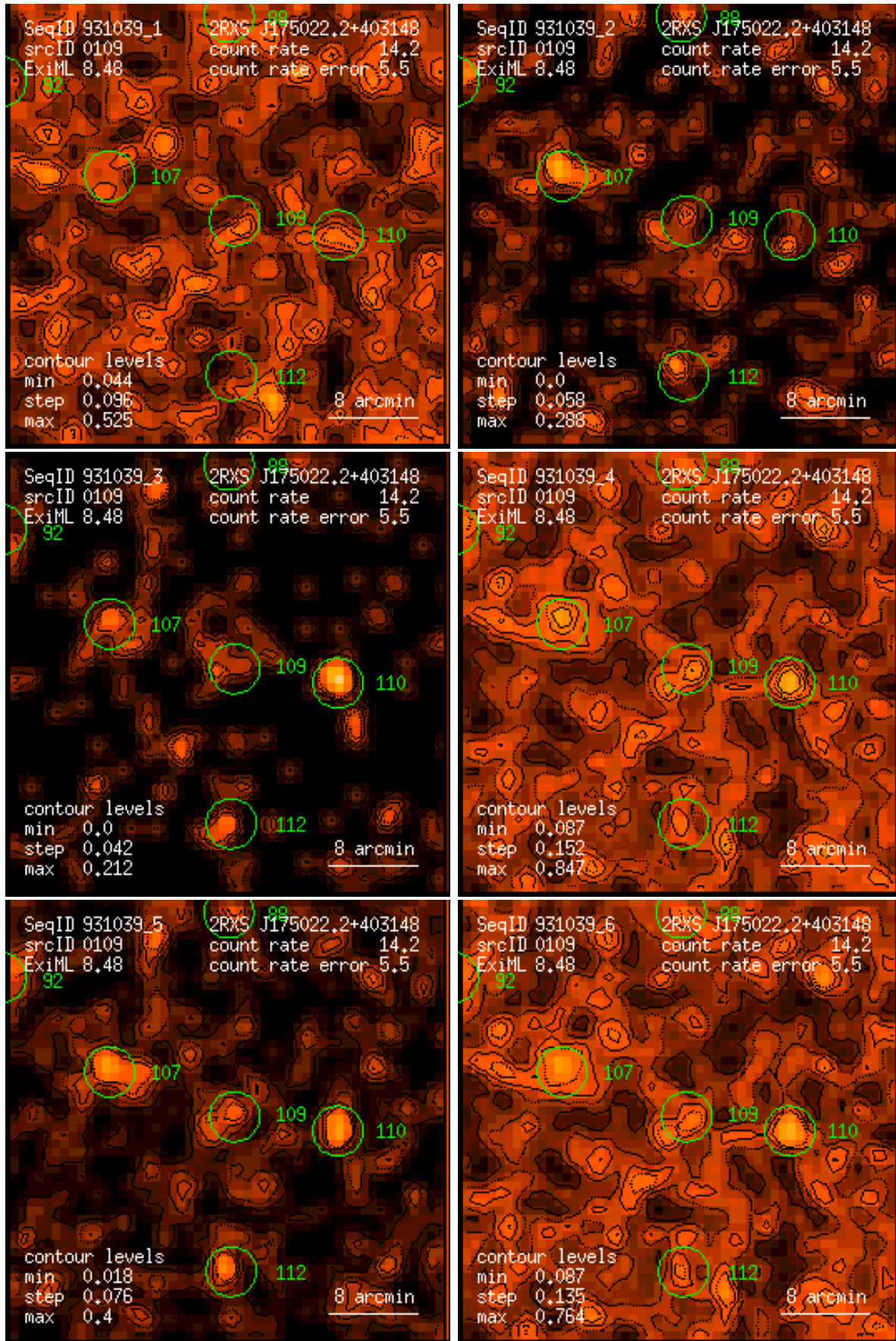
Figure 109: RASS 931039: detection 0109: band rate images, Gaussian filter: (1) PSPC channels 11 – 41, (2) 52 – 90, (3) 91 – 201, (4) 11 – 235, (5) 52 – 201, (6) 11 – 201. Broad band rates in counts/ks. Band rate contour levels in counts/ks/arcmin 2 .
