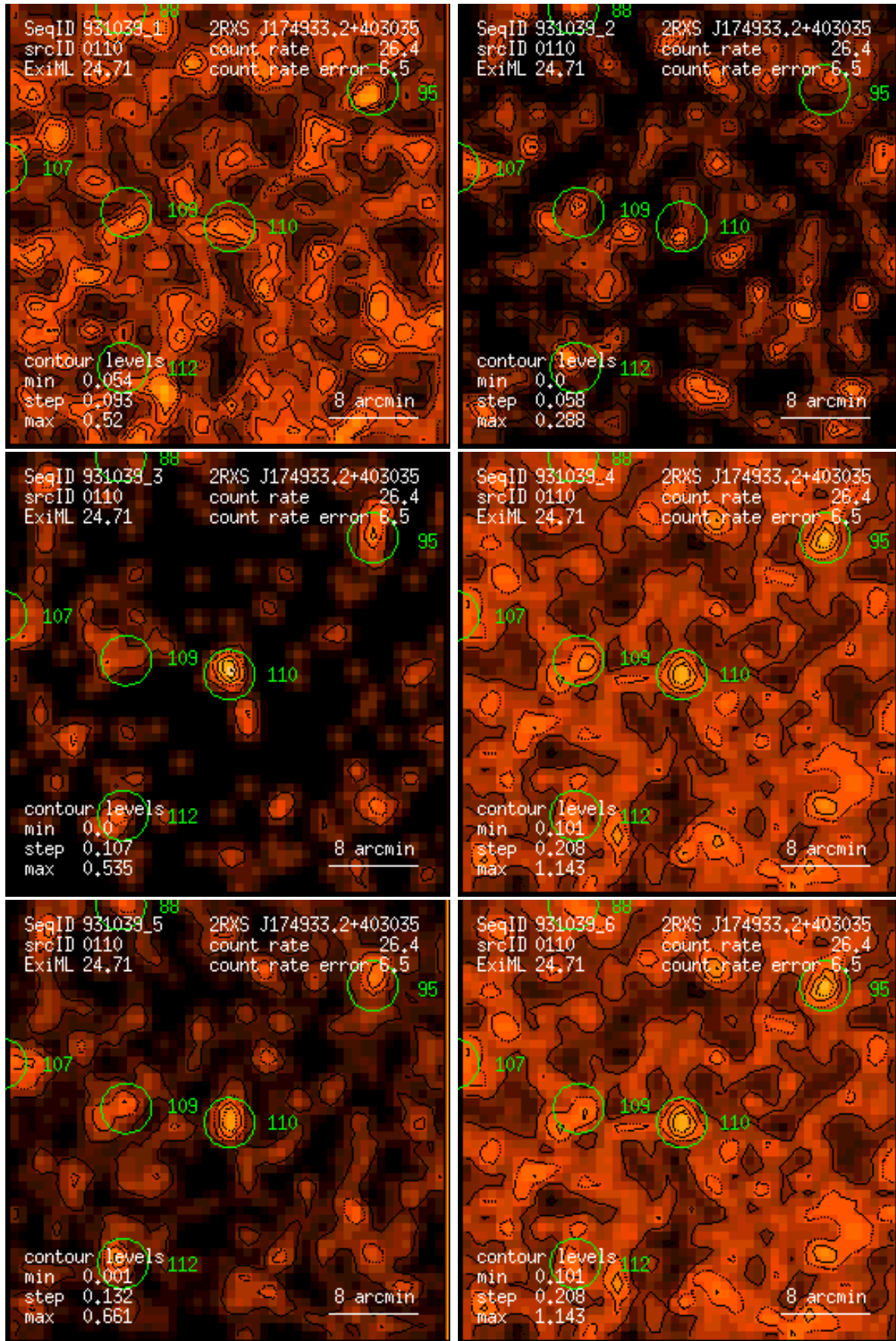
Figure 110: RASS 931039: detection 0110: band rate images, Gaussian filter: (1) PSPC channels 11 – 41, (2) 52 – 90, (3) 91 – 201, (4) 11 – 235, (5) 52 – 201, (6) 11 – 201. Broad band rates in counts/ks. Band rate contour levels in counts/ks/arcmin 2 .
