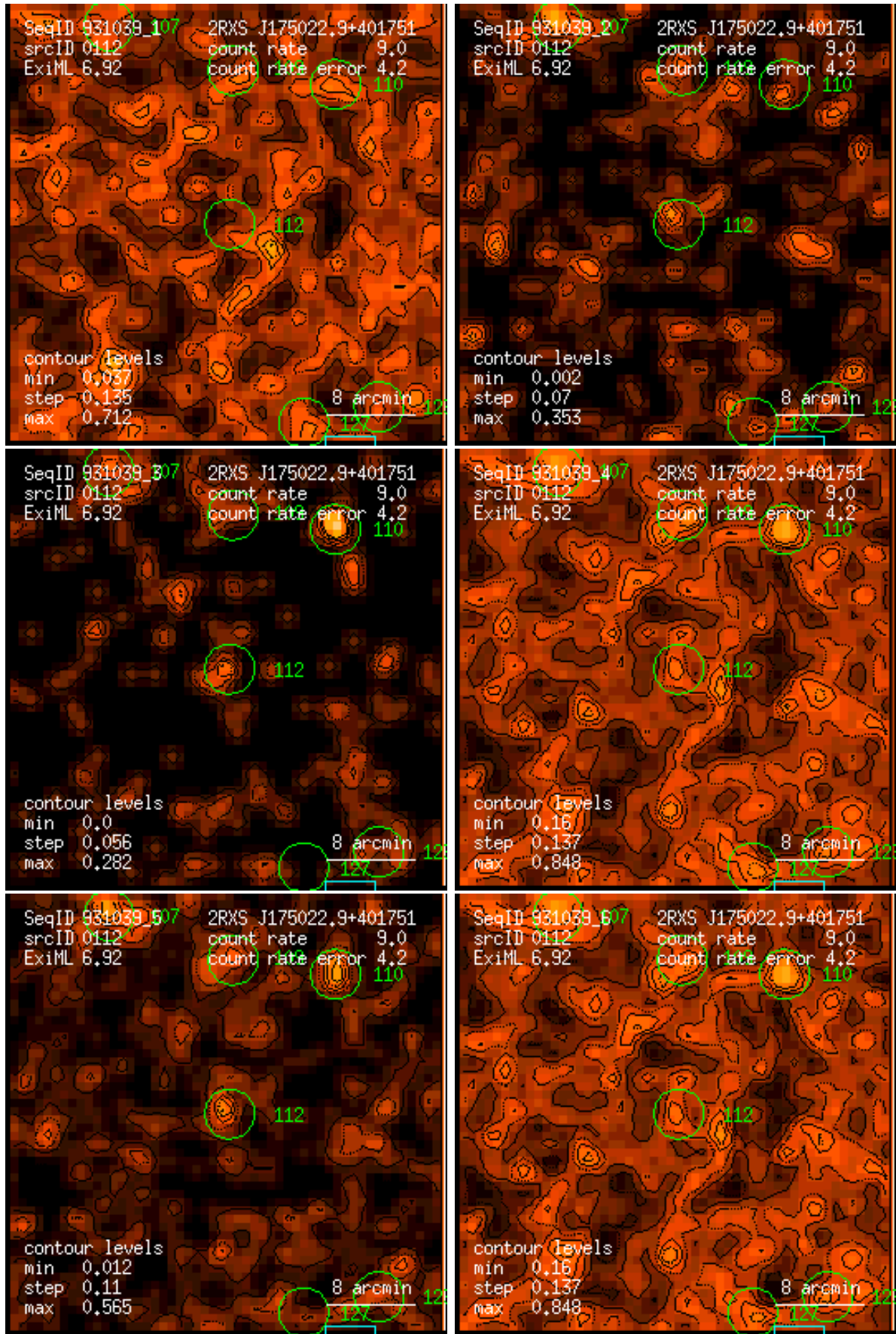
Figure 112: RASS 931039: detection 0112: band rate images, Gaussian filter: (1) PSPC channels 11 – 41, (2) 52 – 90, (3) 91 – 201, (4) 11 – 235, (5) 52 – 201, (6) 11 – 201. Broad band rates in counts/ks. Band rate contour levels in counts/ks/arcmin 2 .
