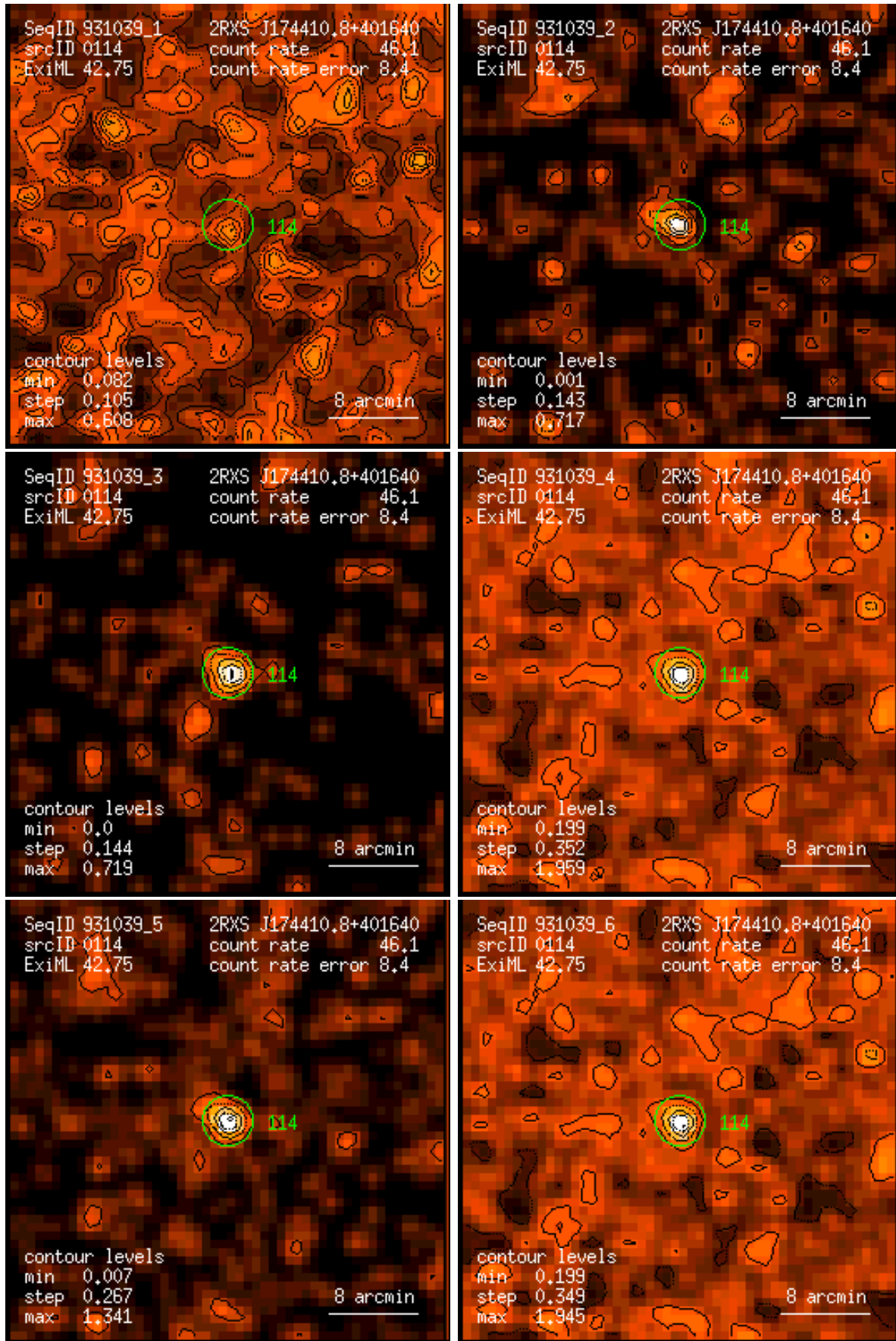
Figure 114: RASS 931039: detection 0114: band rate images, Gaussian filter: (1) PSPC channels 11 – 41, (2) 52 – 90, (3) 91 – 201, (4) 11 – 235, (5) 52 – 201, (6) 11 – 201. Broad band rates in counts/ks. Band rate contour levels in counts/ks/arcmin 2 .
