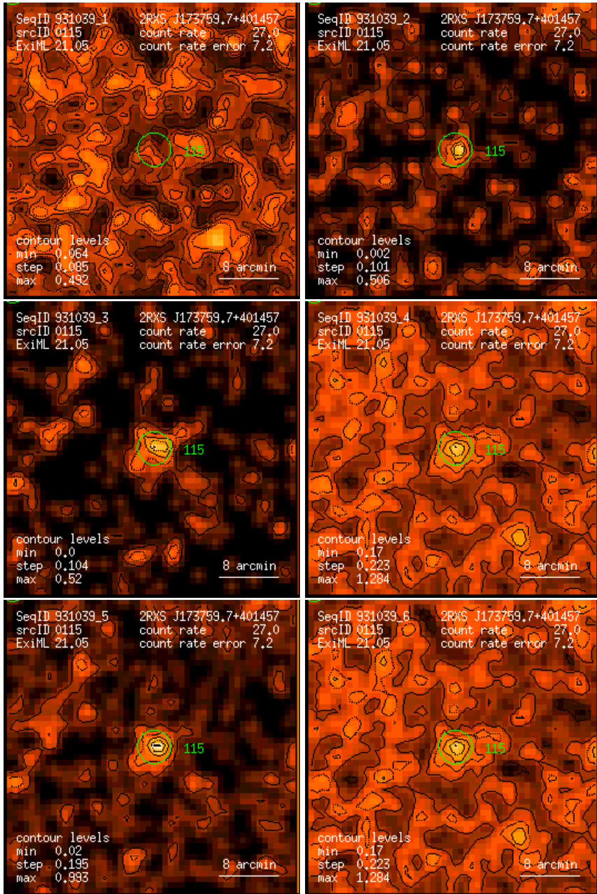
Figure 115: RASS 931039: detection 0115: band rate images, Gaussian filter: (1) PSPC channels 11 – 41, (2) 52 – 90, (3) 91 – 201, (4) 11 – 235, (5) 52 – 201, (6) 11 – 201. Broad band rates in counts/ks. Band rate contour levels in counts/ks/arcmin 2 .
