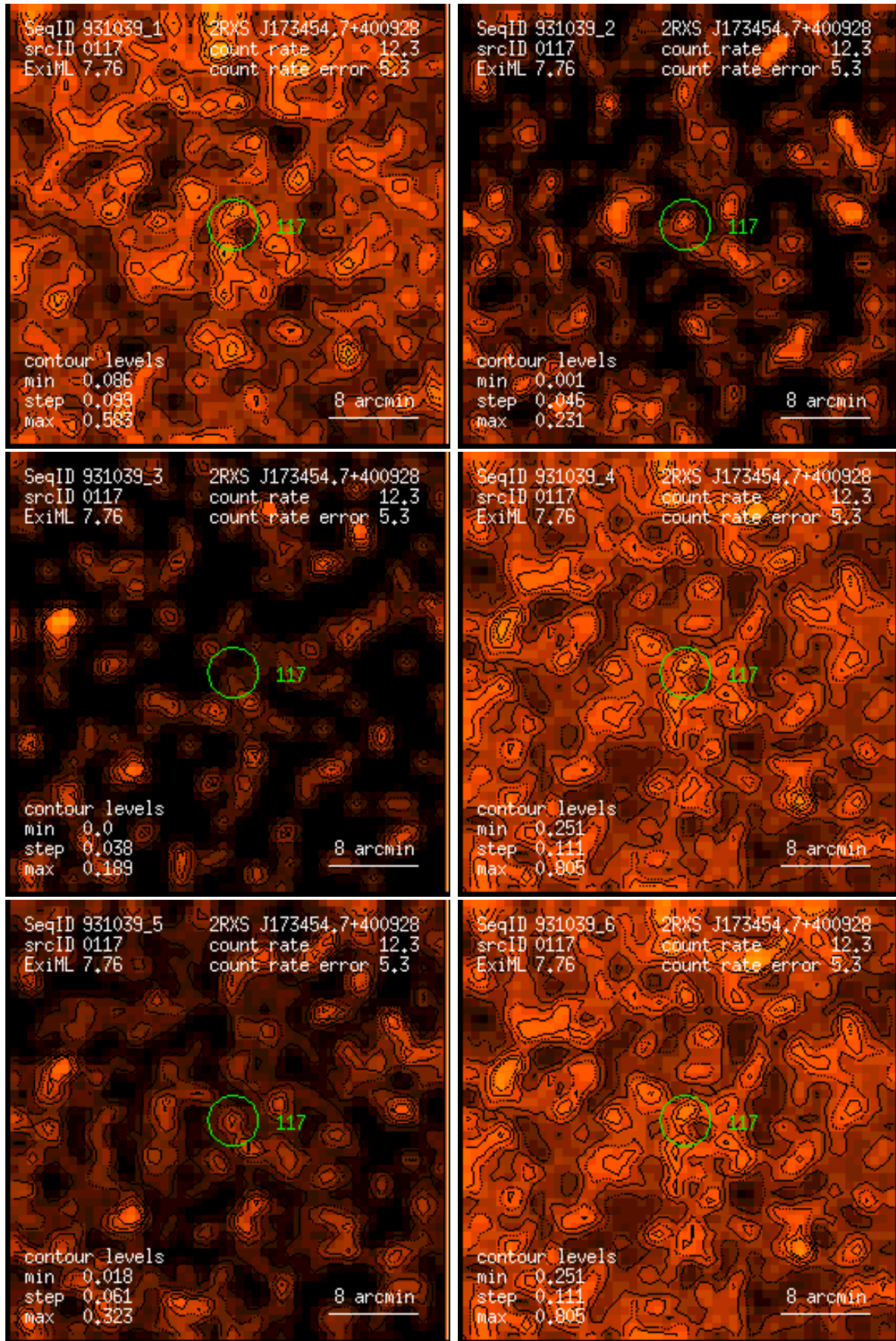
Figure 117: RASS 931039: detection 0117: band rate images, Gaussian filter: (1) PSPC channels 11 – 41, (2) 52 – 90, (3) 91 – 201, (4) 11 – 235, (5) 52 – 201, (6) 11 – 201. Broad band rates in counts/ks. Band rate contour levels in counts/ks/arcmin 2 .
