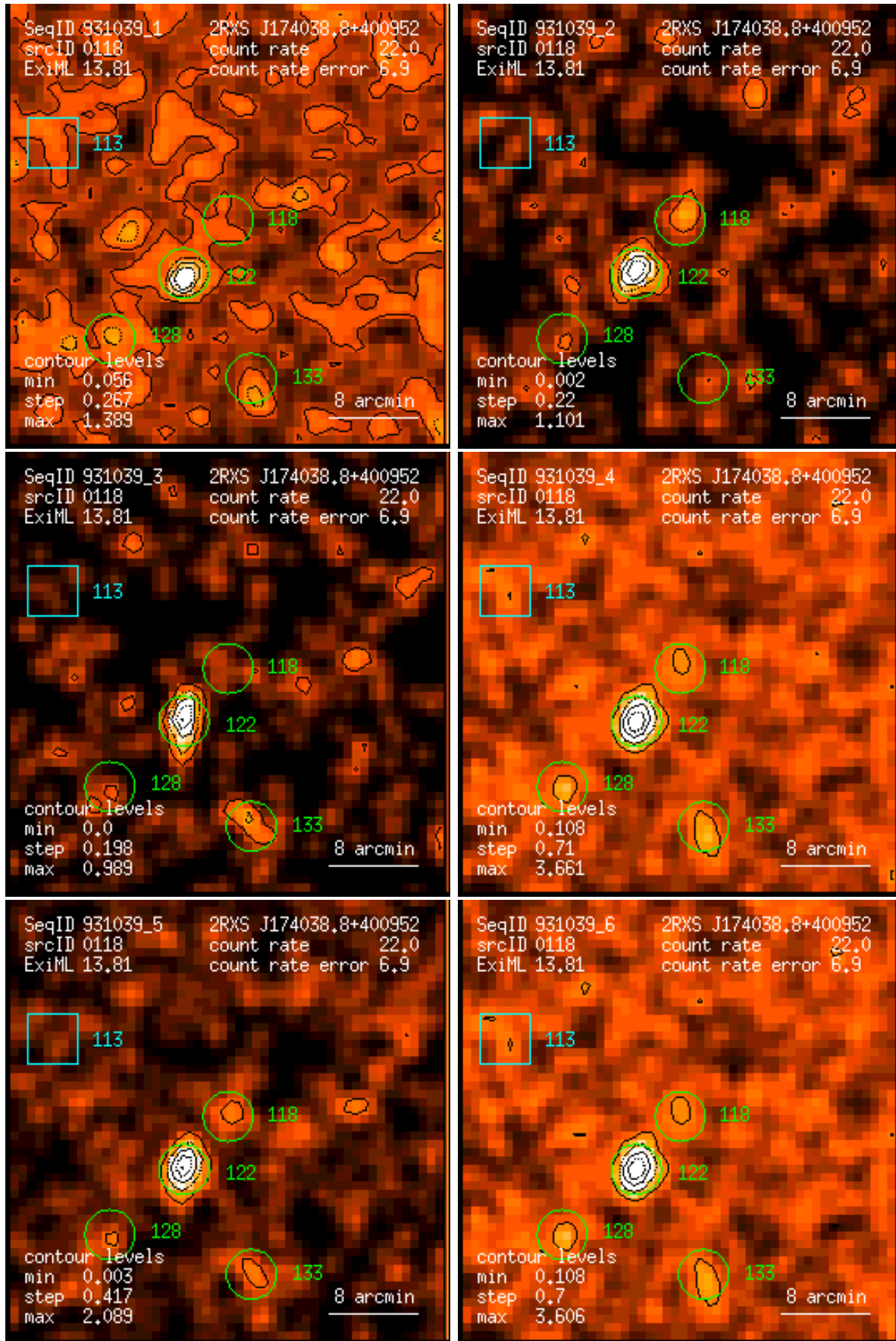
Figure 118: RASS 931039: detection 0118: band rate images, Gaussian filter: (1) PSPC channels 11 – 41, (2) 52 – 90, (3) 91 – 201, (4) 11 – 235, (5) 52 – 201, (6) 11 – 201. Broad band rates in counts/ks. Band rate contour levels in counts/ks/arcmin 2 .
