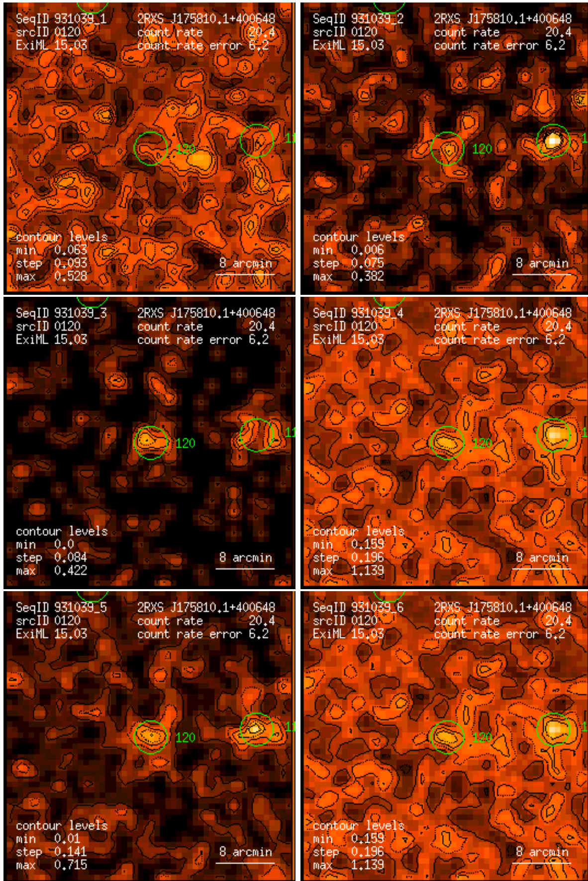
Figure 120: RASS 931039: detection 0120: band rate images, Gaussian filter: (1) PSPC channels 11 – 41, (2) 52 – 90, (3) 91 – 201, (4) 11 – 235, (5) 52 – 201, (6) 11 – 201. Broad band rates in counts/ks. Band rate contour levels in counts/ks/arcmin 2 .
