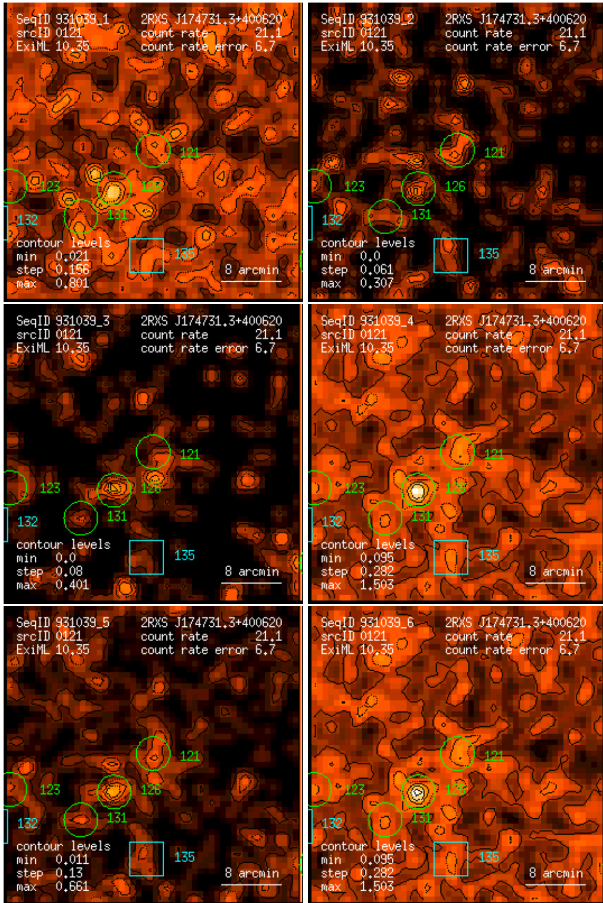
Figure 121: RASS 931039: detection 0121: band rate images, Gaussian filter: (1) PSPC channels 11 – 41, (2) 52 – 90, (3) 91 – 201, (4) 11 – 235, (5) 52 – 201, (6) 11 – 201. Broad band rates in counts/ks. Band rate contour levels in counts/ks/arcmin 2 .
