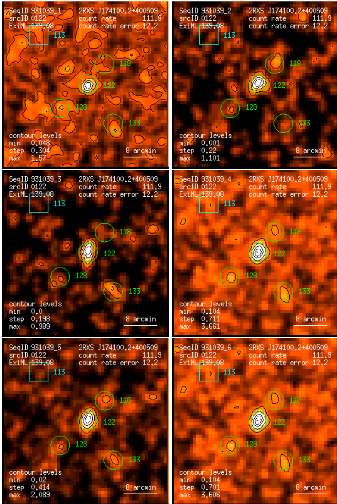
Figure 122: RASS 931039: detection 0122: band rate images, Gaussian filter: (1) PSPC channels 11 – 41, (2) 52 – 90, (3) 91 – 201, (4) 11 – 235, (5) 52 – 201, (6) 11 – 201. Broad band rates in counts/ks. Band rate contour levels in counts/ks/arcmin 2 .
