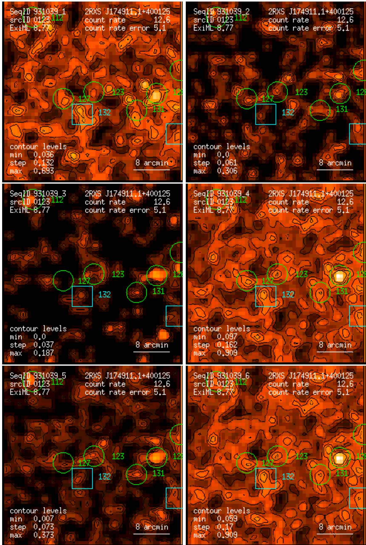
Figure 123: RASS 931039: detection 0123: band rate images, Gaussian filter: (1) PSPC channels 11 – 41, (2) 52 – 90, (3) 91 – 201, (4) 11 – 235, (5) 52 – 201, (6) 11 – 201. Broad band rates in counts/ks. Band rate contour levels in counts/ks/arcmin 2 .
