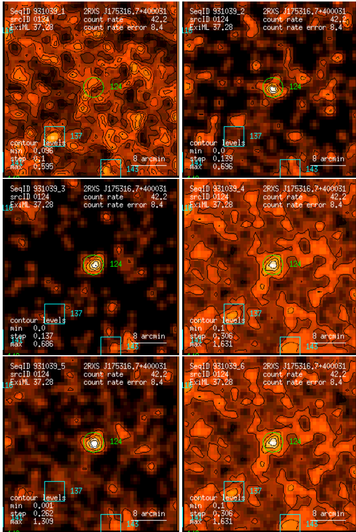
Figure 124: RASS 931039: detection 0124: band rate images, Gaussian filter: (1) PSPC channels 11 – 41, (2) 52 – 90, (3) 91 – 201, (4) 11 – 235, (5) 52 – 201, (6) 11 – 201. Broad band rates in counts/ks. Band rate contour levels in counts/ks/arcmin 2 .
