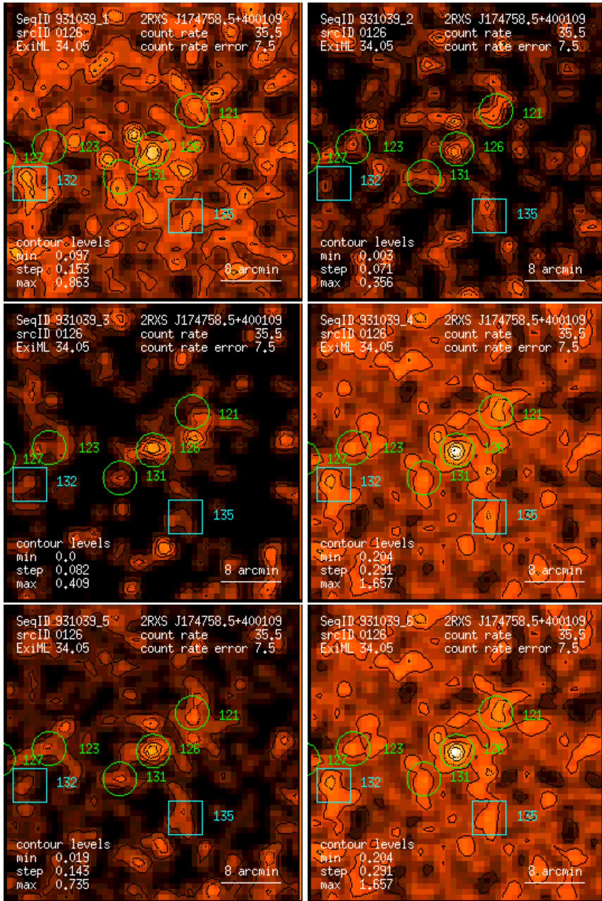
Figure 126: RASS 931039: detection 0126: band rate images, Gaussian filter: (1) PSPC channels 11 – 41, (2) 52 – 90, (3) 91 – 201, (4) 11 – 235, (5) 52 – 201, (6) 11 – 201. Broad band rates in counts/ks. Band rate contour levels in counts/ks/arcmin 2 .
