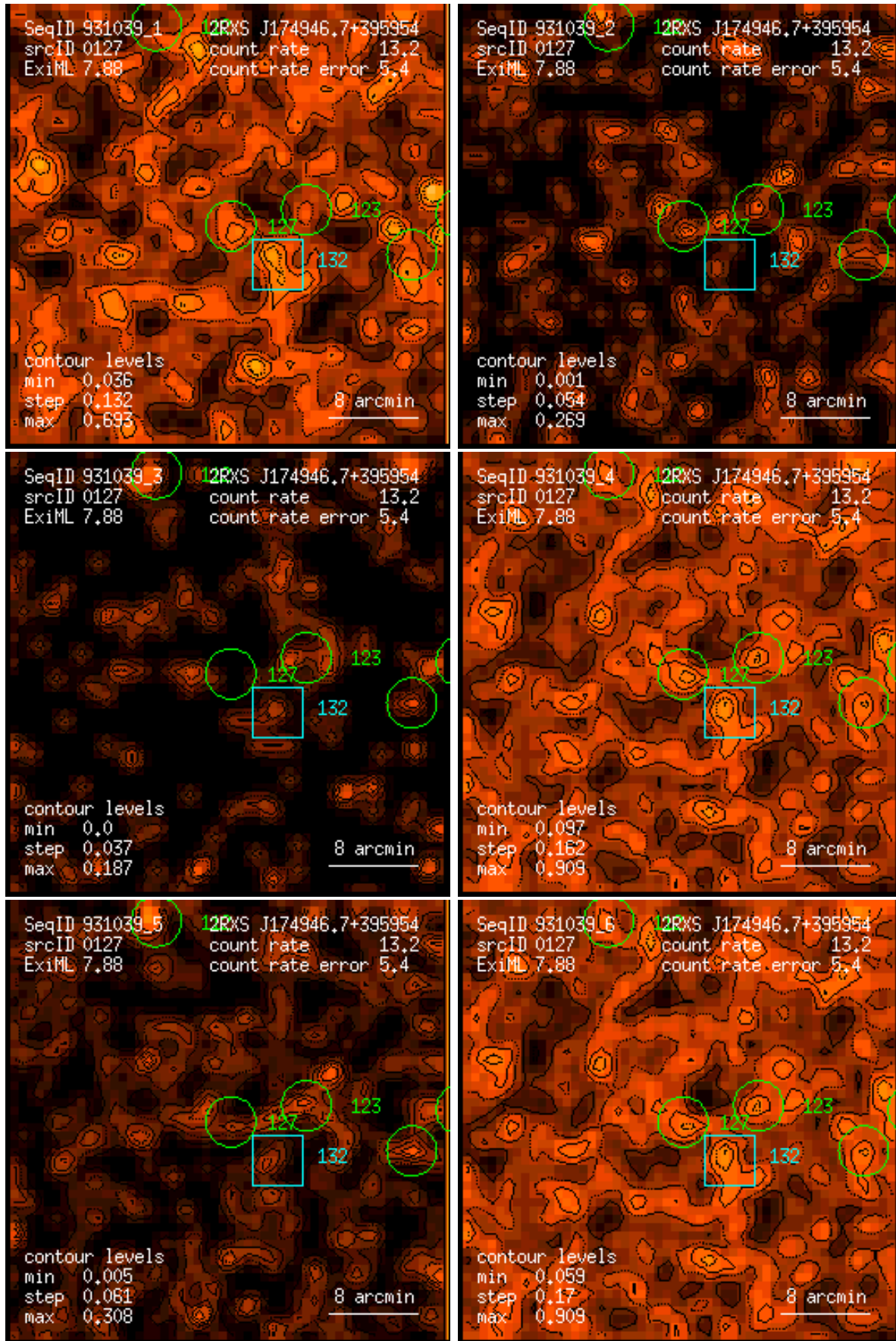
Figure 127: RASS 931039: detection 0127: band rate images, Gaussian filter: (1) PSPC channels 11 – 41, (2) 52 – 90, (3) 91 – 201, (4) 11 – 235, (5) 52 – 201, (6) 11 – 201. Broad band rates in counts/ks. Band rate contour levels in counts/ks/arcmin 2 .
