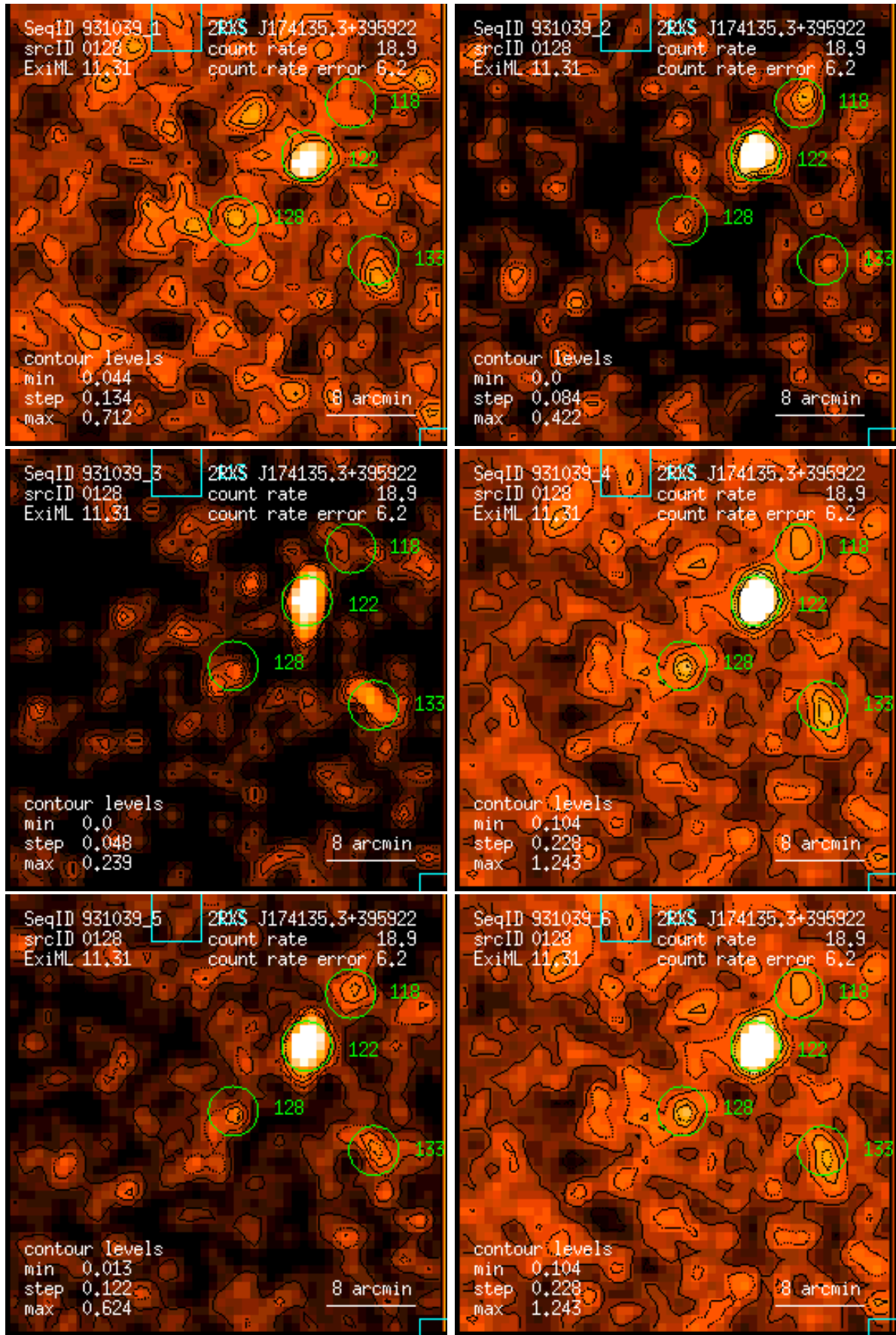
Figure 128: RASS 931039: detection 0128: band rate images, Gaussian filter: (1) PSPC channels 11 – 41, (2) 52 – 90, (3) 91 – 201, (4) 11 – 235, (5) 52 – 201, (6) 11 – 201. Broad band rates in counts/ks. Band rate contour levels in counts/ks/arcmin 2 .
