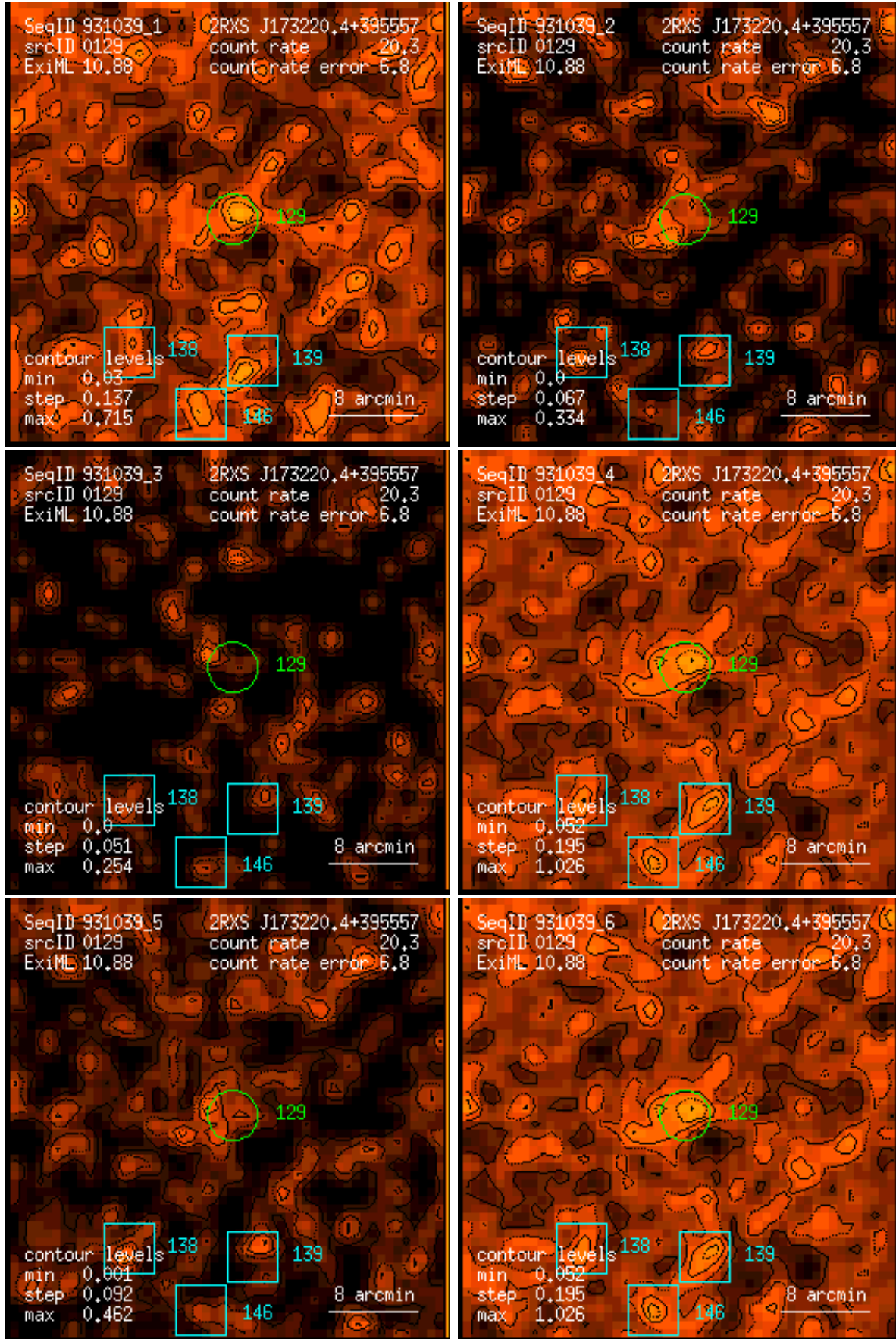
Figure 129: RASS 931039: detection 0129: band rate images, Gaussian filter: (1) PSPC channels 11 – 41, (2) 52 – 90, (3) 91 – 201, (4) 11 – 235, (5) 52 – 201, (6) 11 – 201. Broad band rates in counts/ks. Band rate contour levels in counts/ks/arcmin 2 .
