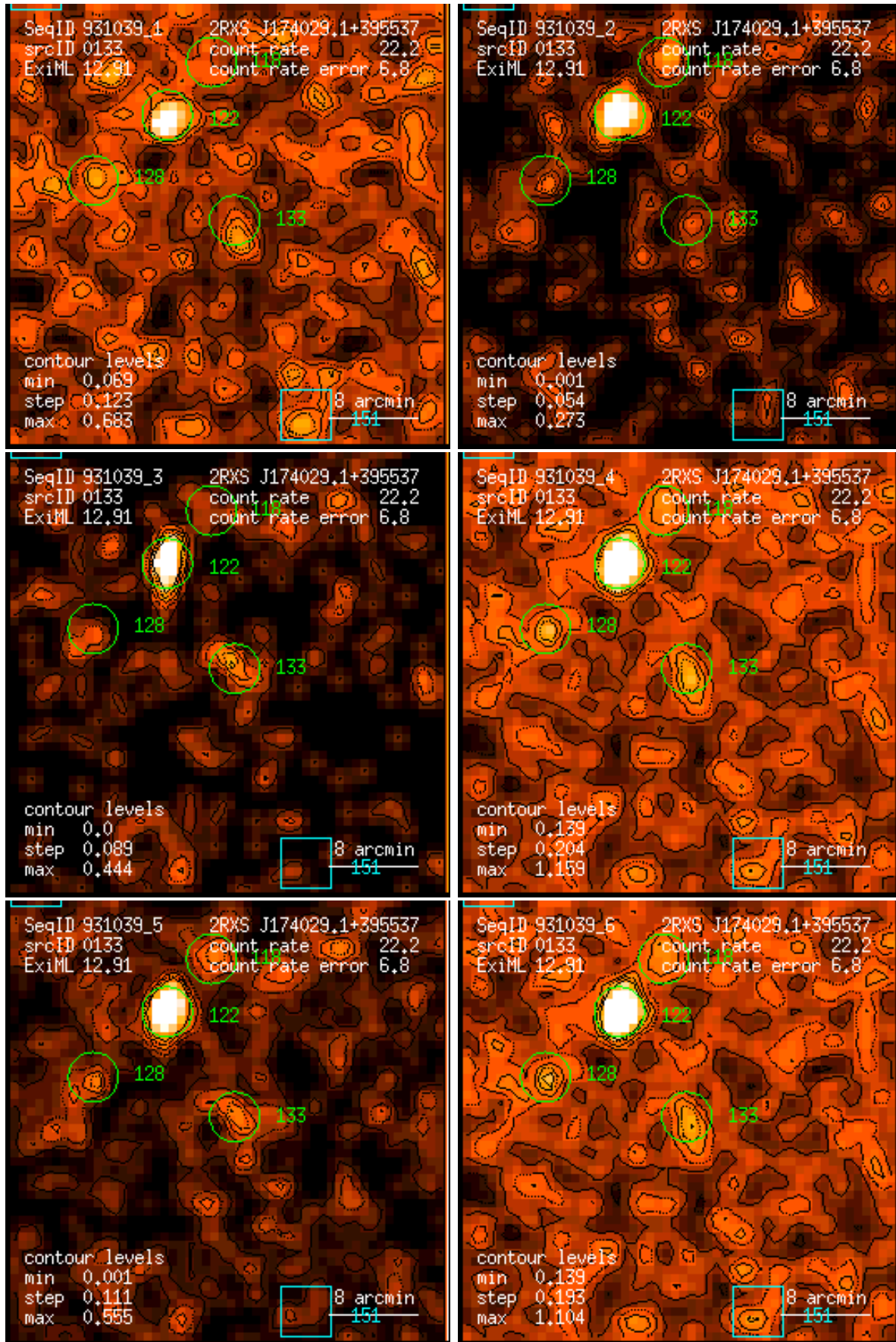
Figure 133: RASS 931039: detection 0133: band rate images, Gaussian filter: (1) PSPC channels 11 – 41, (2) 52 – 90, (3) 91 – 201, (4) 11 – 235, (5) 52 – 201, (6) 11 – 201. Broad band rates in counts/ks. Band rate contour levels in counts/ks/arcmin 2 .
