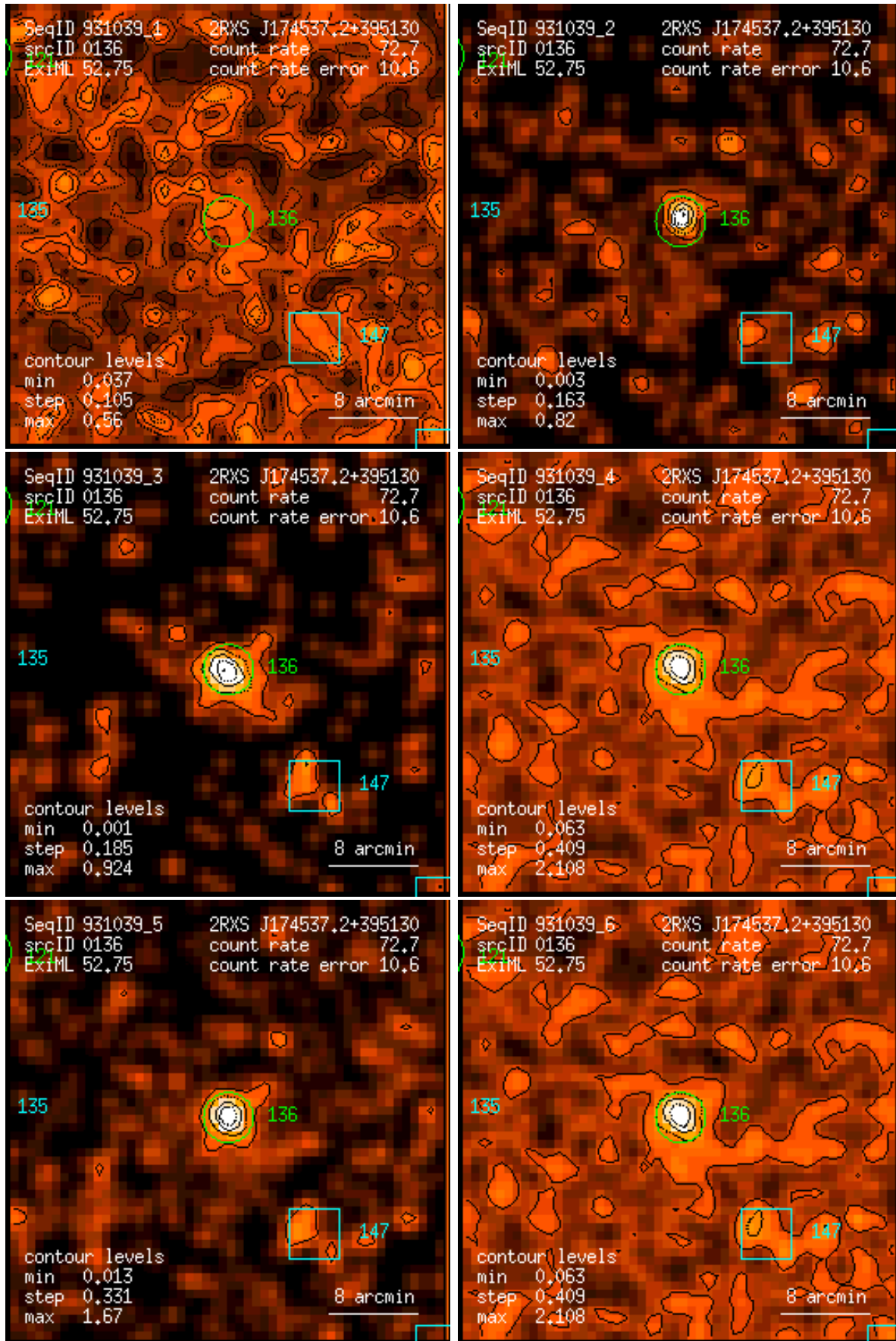
Figure 136: RASS 931039: detection 0136: band rate images, Gaussian filter: (1) PSPC channels 11 – 41, (2) 52 – 90, (3) 91 – 201, (4) 11 – 235, (5) 52 – 201, (6) 11 – 201. Broad band rates in counts/ks. Band rate contour levels in counts/ks/arcmin 2 .
