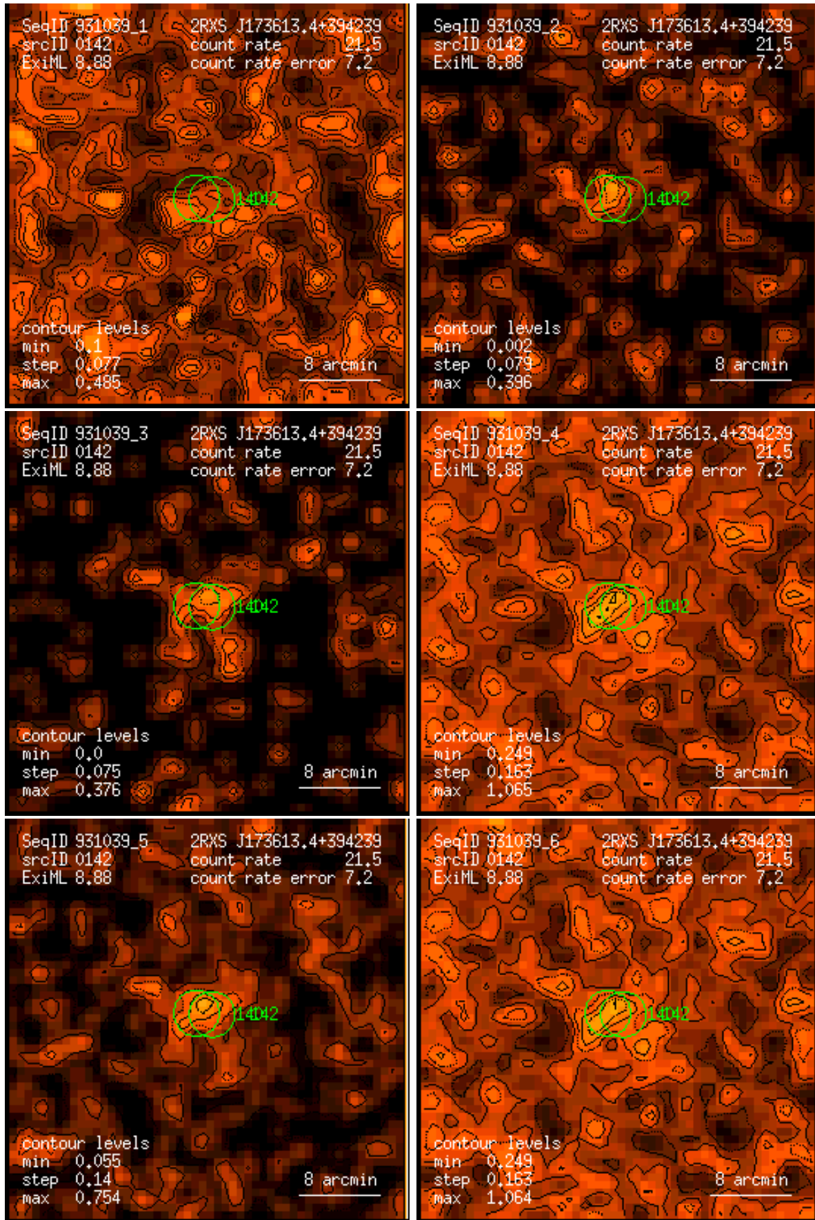
Figure 142: RASS 931039: detection 0142: band rate images, Gaussian filter: (1) PSPC channels 11 – 41, (2) 52 – 90, (3) 91 – 201, (4) 11 – 235, (5) 52 – 201, (6) 11 – 201. Broad band rates in counts/ks. Band rate contour levels in counts/ks/arcmin 2 .
