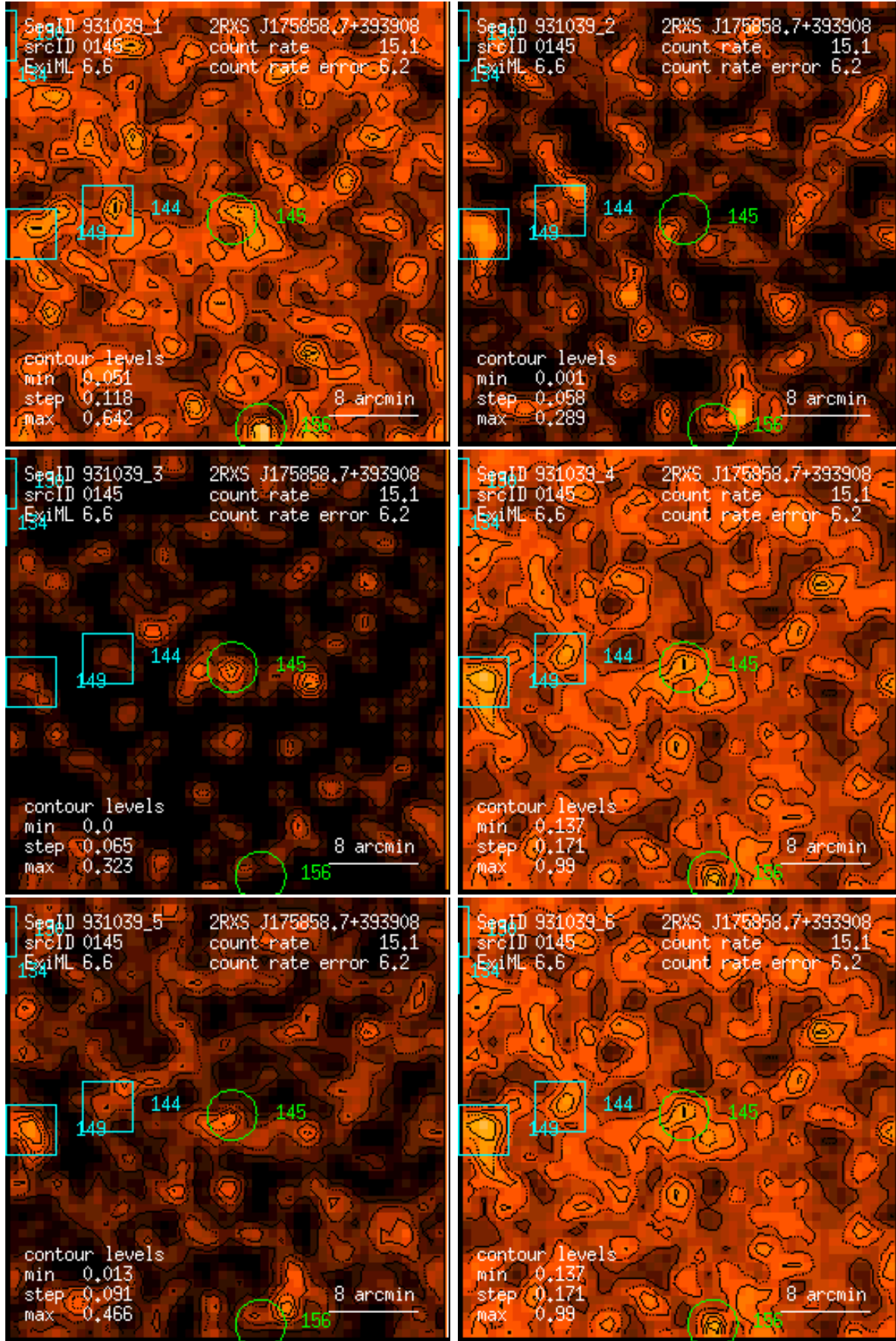
Figure 145: RASS 931039: detection 0145: band rate images, Gaussian filter: (1) PSPC channels 11 – 41, (2) 52 – 90, (3) 91 – 201, (4) 11 – 235, (5) 52 – 201, (6) 11 – 201. Broad band rates in counts/ks. Band rate contour levels in counts/ks/arcmin 2 .
