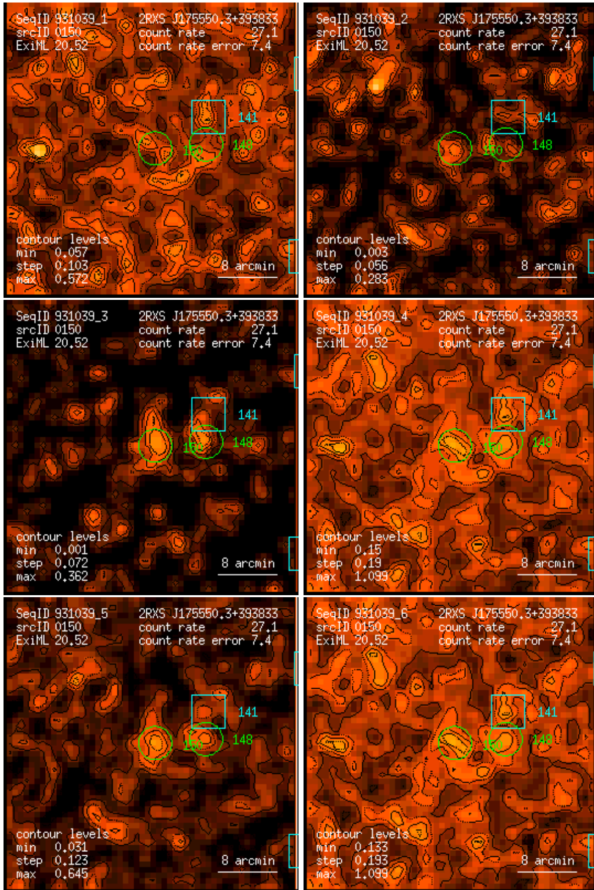
Figure 150: RASS 931039: detection 0150: band rate images, Gaussian filter: (1) PSPC channels 11 – 41, (2) 52 – 90, (3) 91 – 201, (4) 11 – 235, (5) 52 – 201, (6) 11 – 201. Broad band rates in counts/ks. Band rate contour levels in counts/ks/arcmin 2 .
