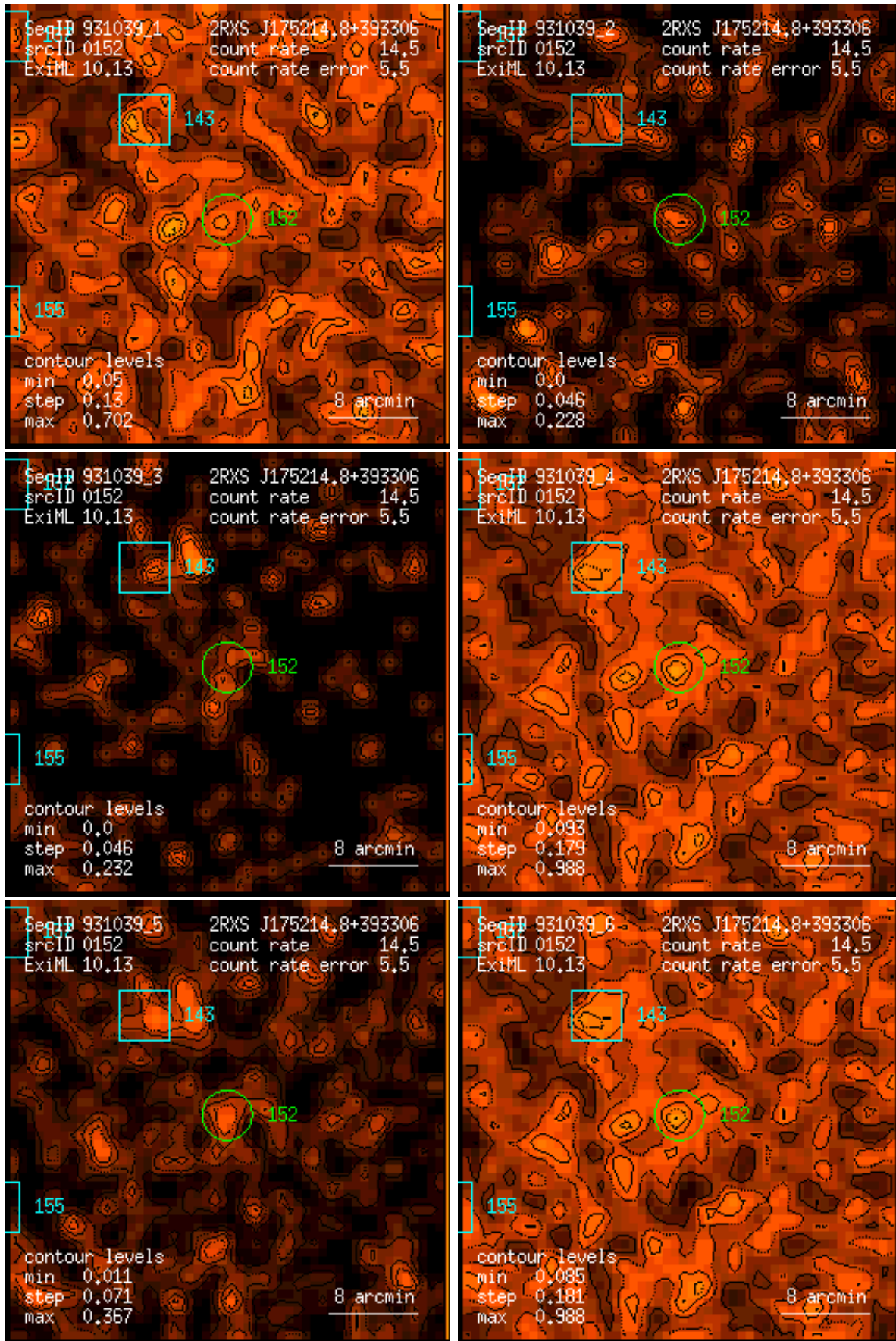
Figure 152: RASS 931039: detection 0152: band rate images, Gaussian filter: (1) PSPC channels 11 – 41, (2) 52 – 90, (3) 91 – 201, (4) 11 – 235, (5) 52 – 201, (6) 11 – 201. Broad band rates in counts/ks. Band rate contour levels in counts/ks/arcmin 2 .
