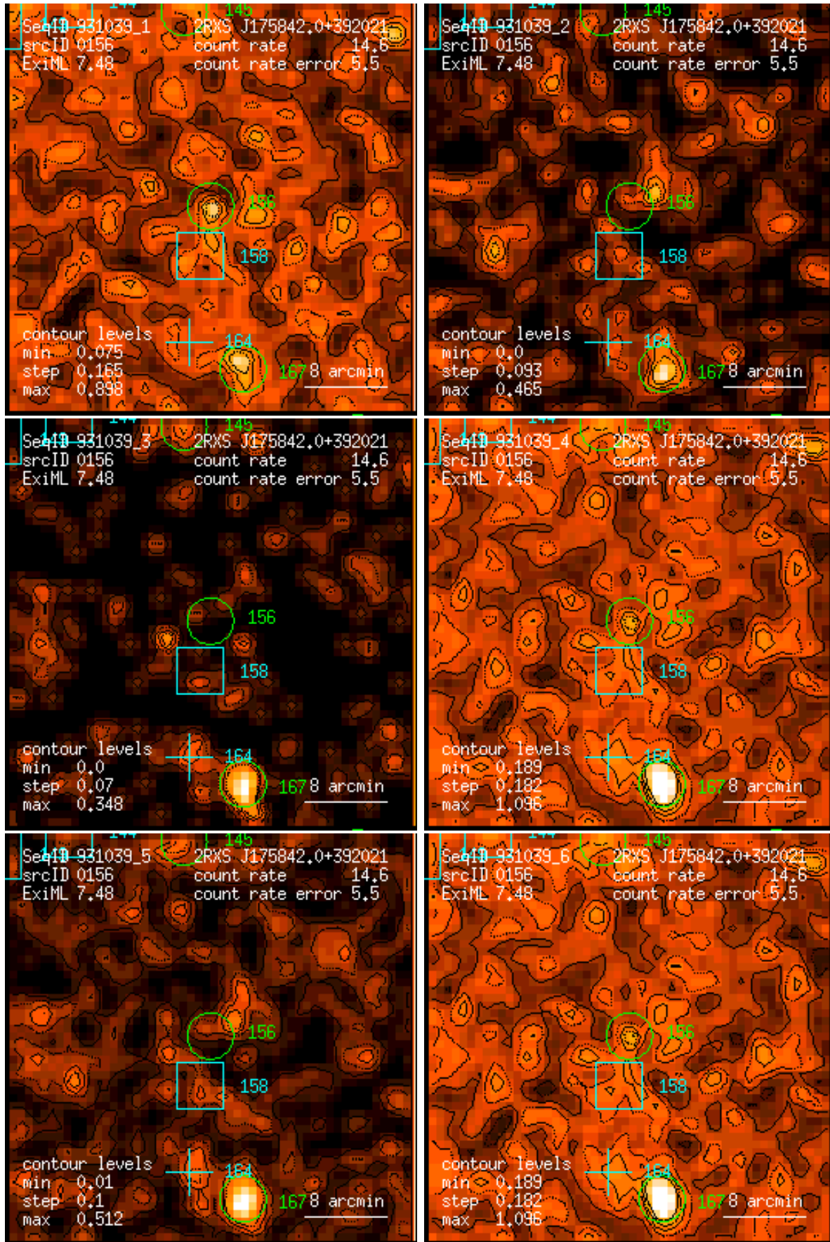
Figure 156: RASS 931039: detection 0156: band rate images, Gaussian filter: (1) PSPC channels 11 – 41, (2) 52 – 90, (3) 91 – 201, (4) 11 – 235, (5) 52 – 201, (6) 11 – 201. Broad band rates in counts/ks. Band rate contour levels in counts/ks/arcmin 2 .
