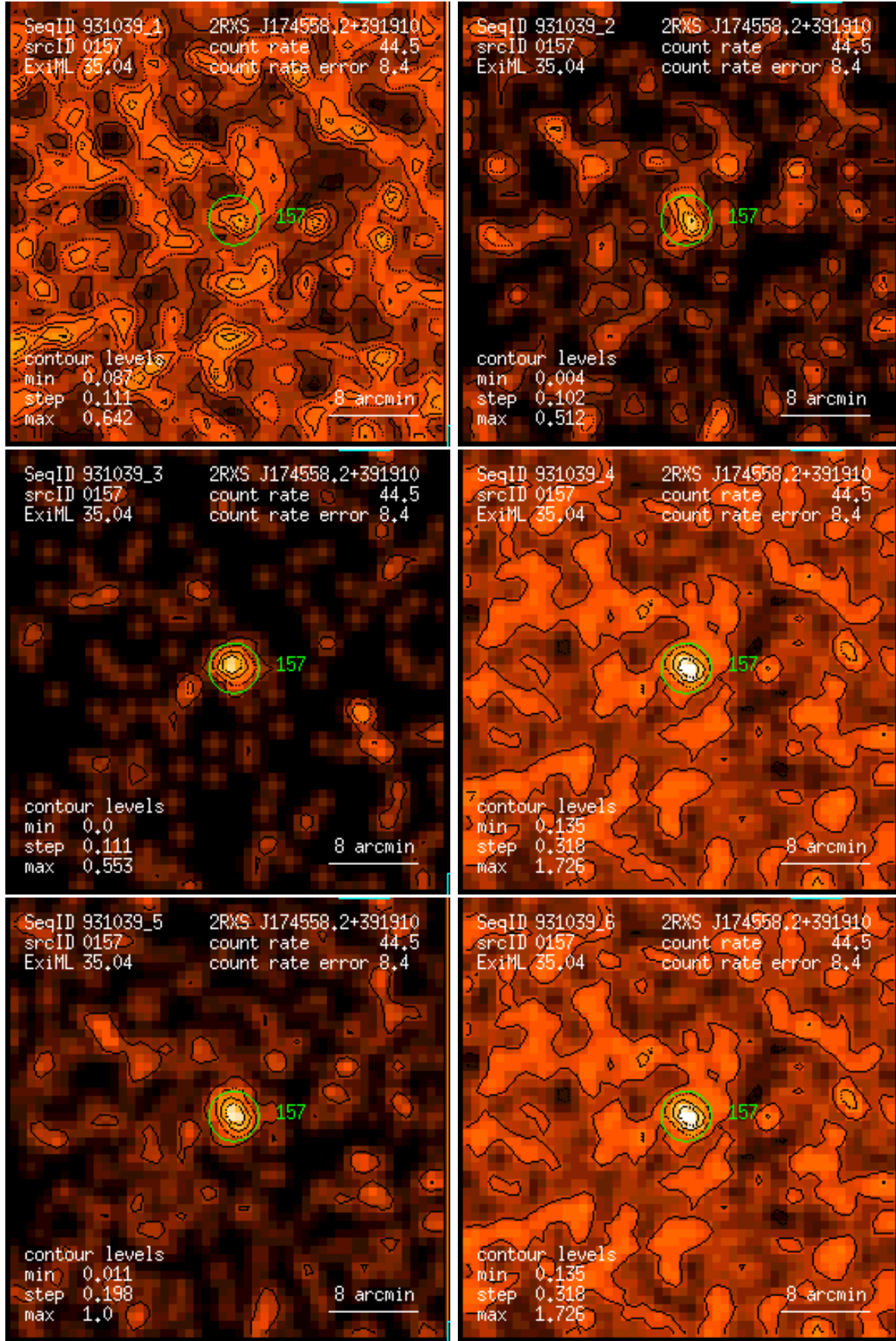
Figure 157: RASS 931039: detection 0157: band rate images, Gaussian filter: (1) PSPC channels 11 – 41, (2) 52 – 90, (3) 91 – 201, (4) 11 – 235, (5) 52 – 201, (6) 11 – 201. Broad band rates in counts/ks. Band rate contour levels in counts/ks/arcmin 2 .
