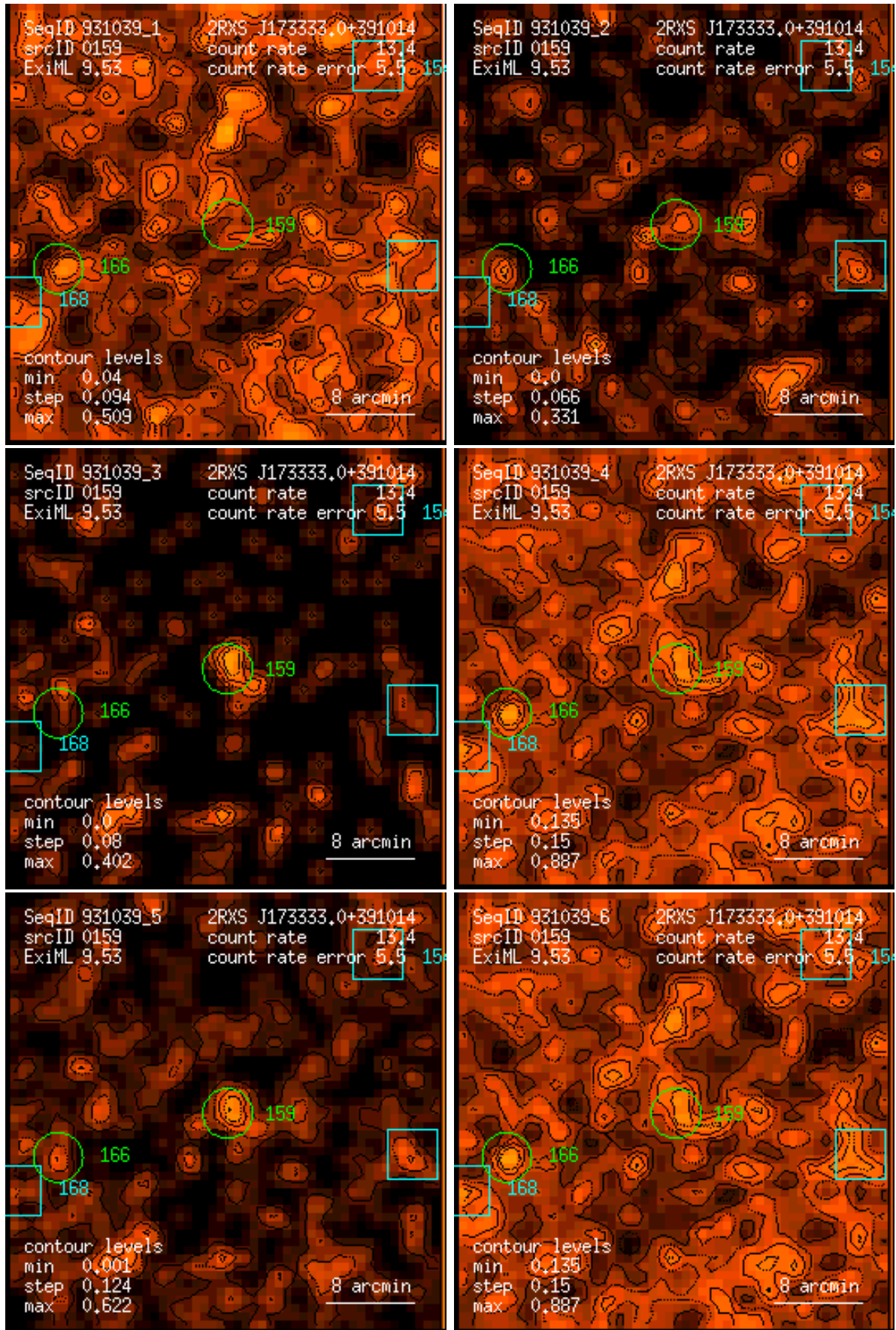
Figure 159: RASS 931039: detection 0159: band rate images, Gaussian filter: (1) PSPC channels 11 – 41, (2) 52 – 90, (3) 91 – 201, (4) 11 – 235, (5) 52 – 201, (6) 11 – 201. Broad band rates in counts/ks. Band rate contour levels in counts/ks/arcmin 2 .
