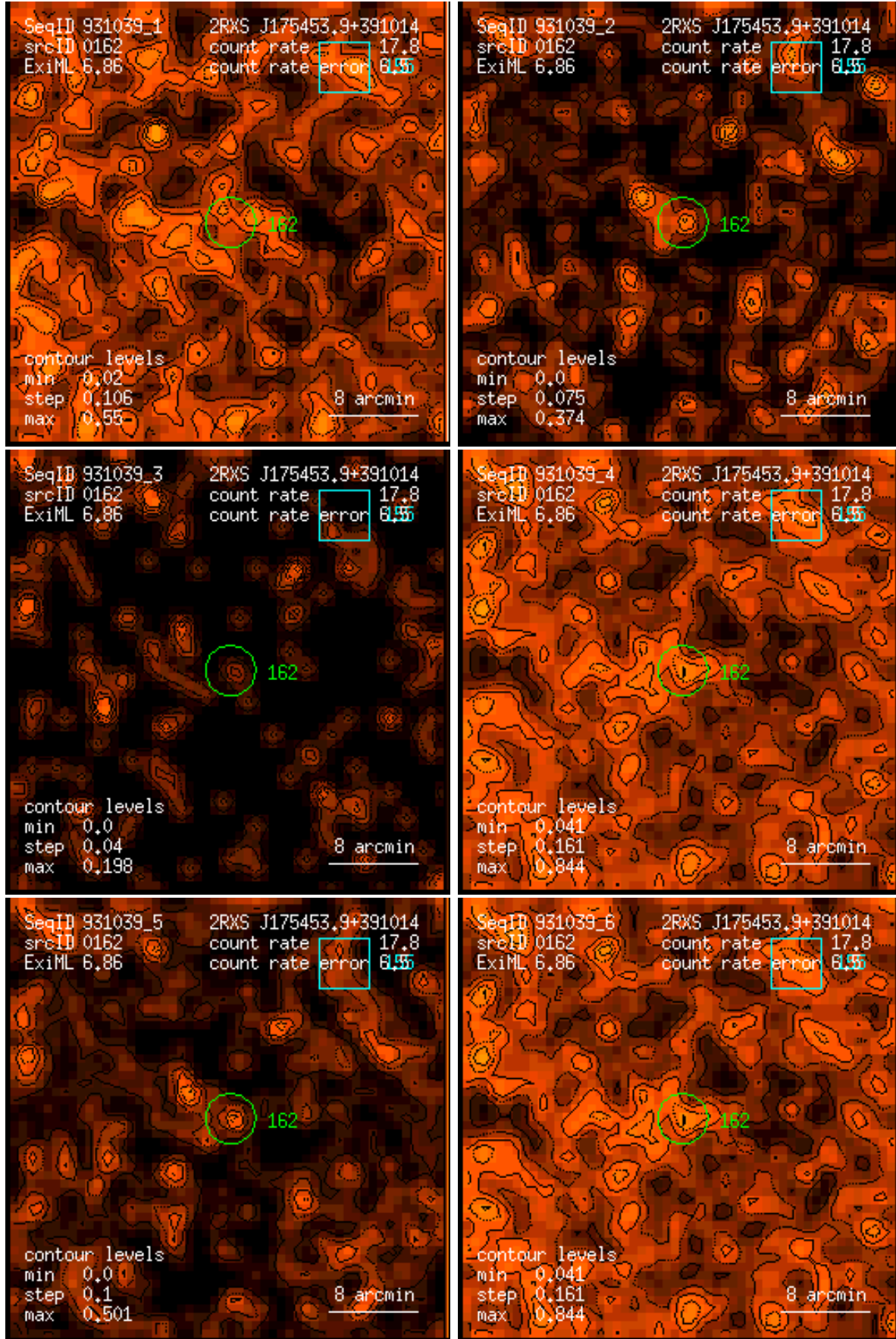
Figure 162: RASS 931039: detection 0162: band rate images, Gaussian filter: (1) PSPC channels 11 – 41, (2) 52 – 90, (3) 91 – 201, (4) 11 – 235, (5) 52 – 201, (6) 11 – 201. Broad band rates in counts/ks. Band rate contour levels in counts/ks/arcmin 2 .
