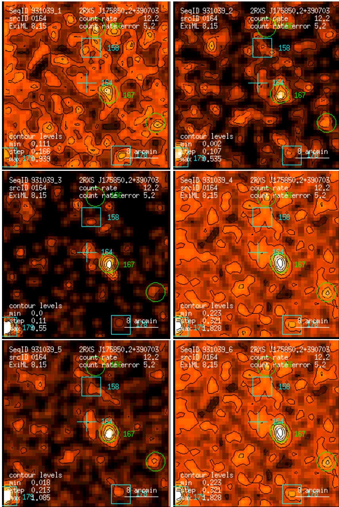
Figure 164: RASS 931039: detection 0164: band rate images, Gaussian filter: (1) PSPC channels 11 – 41, (2) 52 – 90, (3) 91 – 201, (4) 11 – 235, (5) 52 – 201, (6) 11 – 201. Broad band rates in counts/ks. Band rate contour levels in counts/ks/arcmin 2 .
