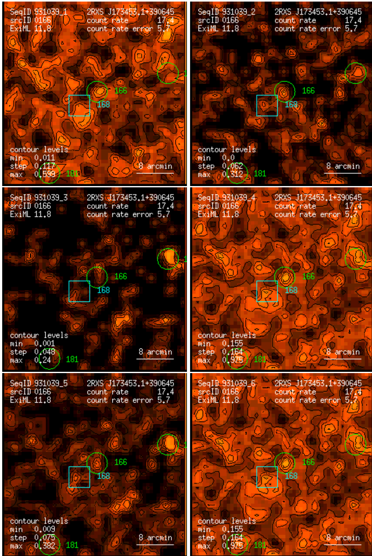
Figure 166: RASS 931039: detection 0166: band rate images, Gaussian filter: (1) PSPC channels 11 – 41, (2) 52 – 90, (3) 91 – 201, (4) 11 – 235, (5) 52 – 201, (6) 11 – 201. Broad band rates in counts/ks. Band rate contour levels in counts/ks/arcmin 2 .
