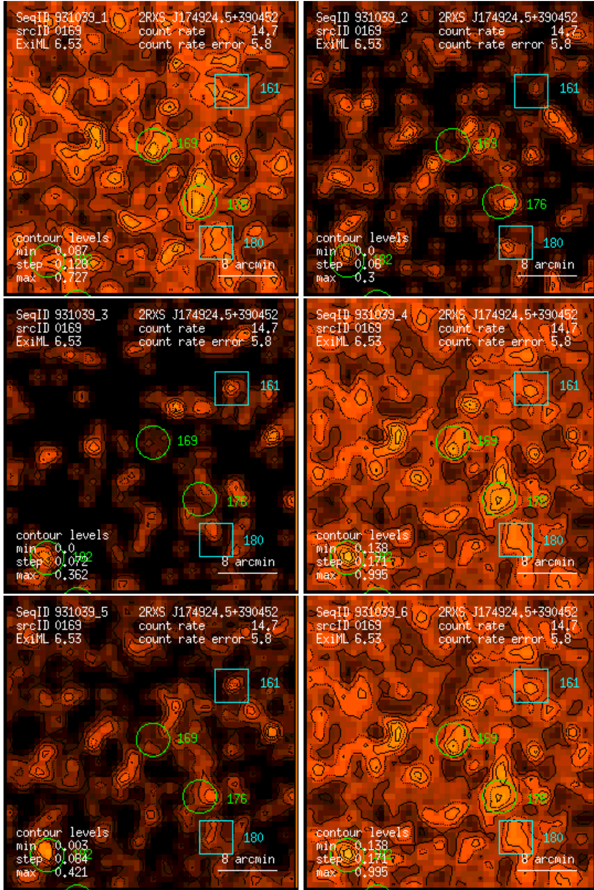
Figure 169: RASS 931039: detection 0169: band rate images, Gaussian filter: (1) PSPC channels 11 – 41, (2) 52 – 90, (3) 91 – 201, (4) 11 – 235, (5) 52 – 201, (6) 11 – 201. Broad band rates in counts/ks. Band rate contour levels in counts/ks/arcmin 2 .
